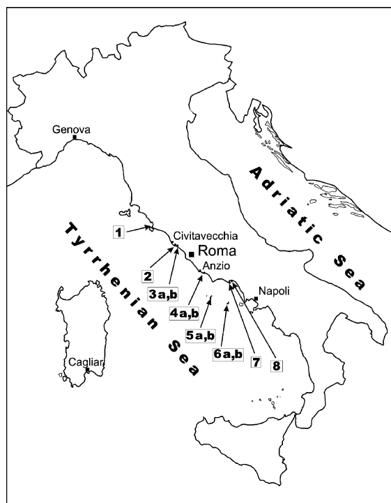
Fig. 1. Location map of the Roman epoch piscinae and tide-gauge sites along the central Tyrrhenian coast of Italy: (1) Santa Liberata, (2) Punta della Vipera, (3a) Santa Marinella Odescalchi, (3b) Santa Marinella Le Grottacce, (4a) La Banca, (4b) Torre Astura, (5a,b) Ponza (outdoor and indoor fish tank), (6a,b) Ventotene harbour and fish tanks, (7) Serapo and (8) Sarinola. The four tide gauge sites are located at Genova, Civitavecchia, Naples and Cagliari.
