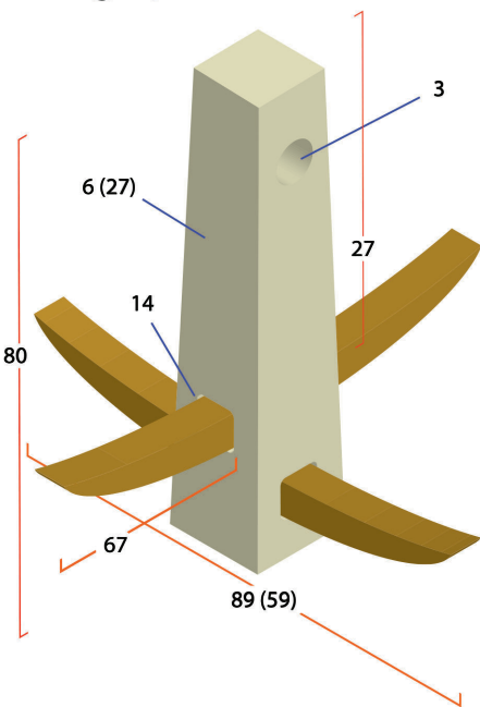
Stone-frame grapnel-anchor
