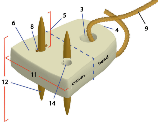
Stone-frame staked anchor
