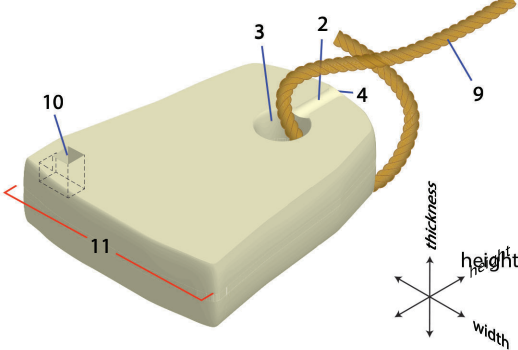
Pierced stone anchor
