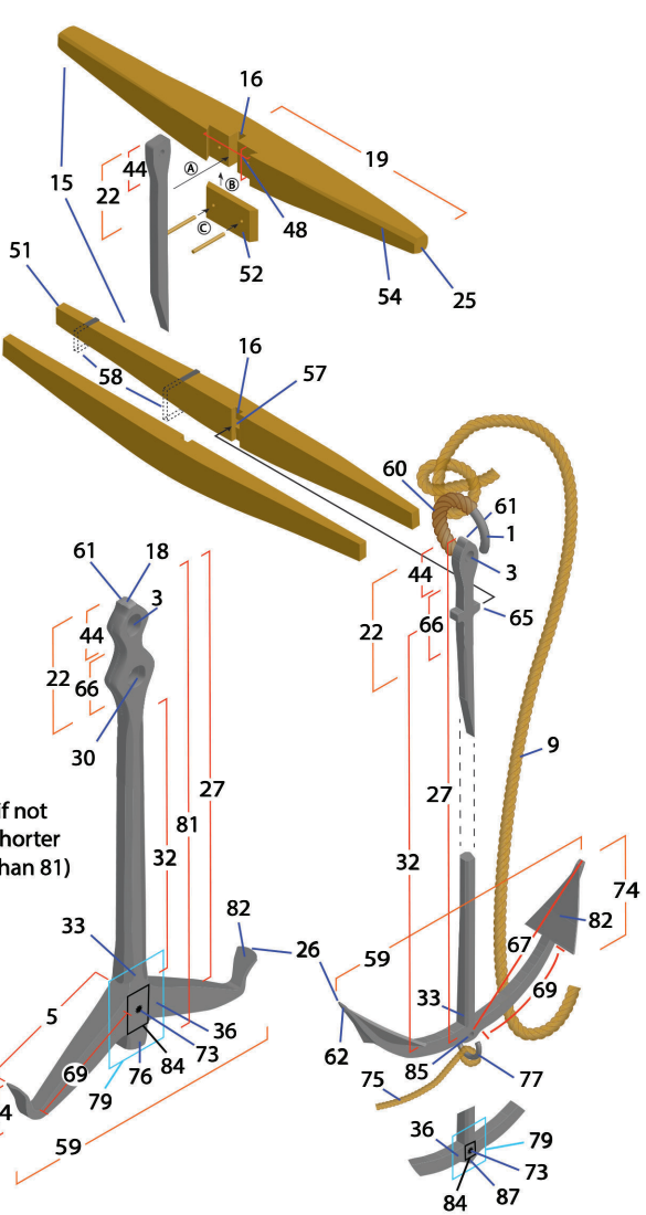
Iron frame wood-stock-anchor
