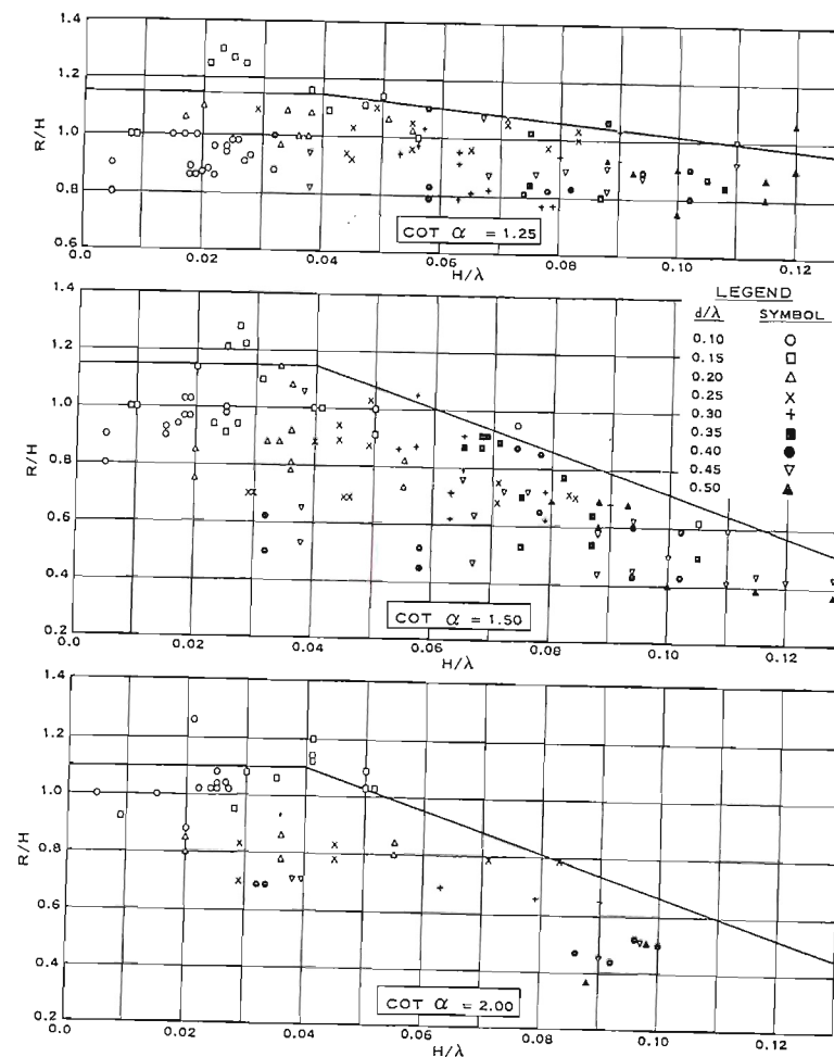
FIG. 6.—WAVE RUN-UP ON RUBBLE-MOUND BREAKWATERS: R/H = f(H/\lambda, d/\lambda)
