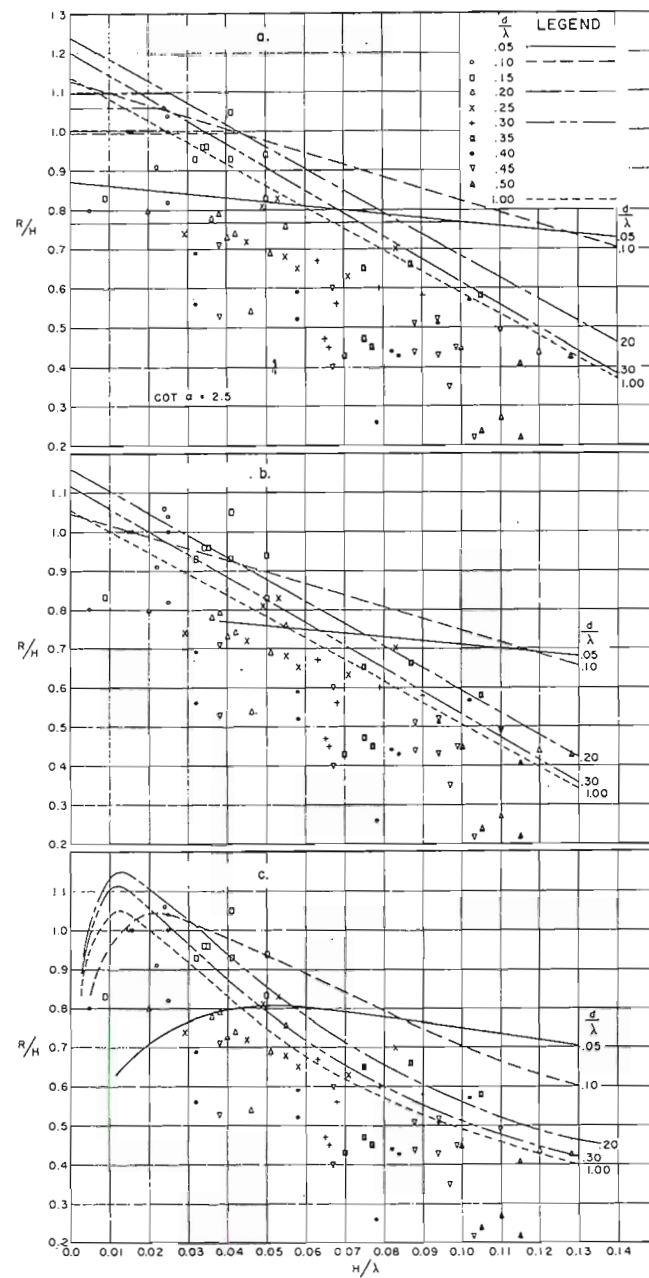
FIG. 13.—WAVE RUN-UP ON RUBBLE SLOPE, 1 ON 2.5. RELATIONSHIP TO RELATIVE DEPTH FOR SEVERAL POSSIBLE RUN-UP CURVES
