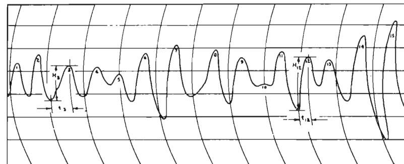
FIG. 9.—TYPICAL SECTION OF A WAVE RECORD
