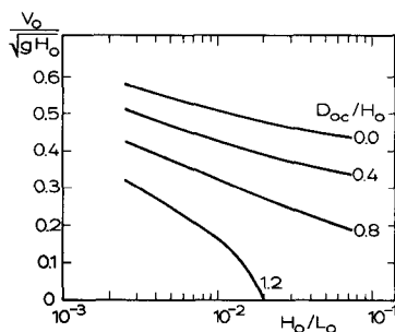
Figure 5.20 The scale for the longshore current velocity V_0 as a function of the depth at the crest of the bar and the deep water steepness.
