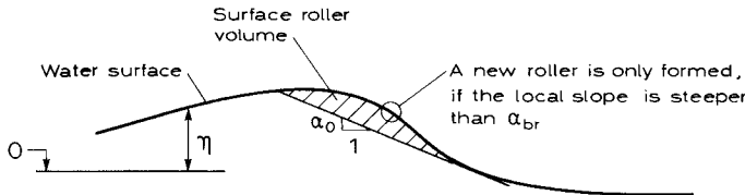
Figure 4.19 Principles for determining the geometry of the surface roller.
