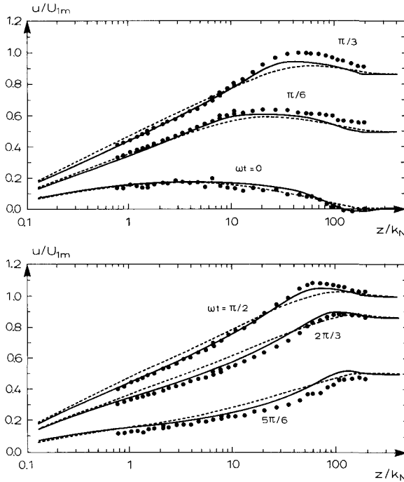
Figure 2.21 Calculated and measured flow velocity. a/k_N = 3700 . Symbols as in Fig. 2.18.
