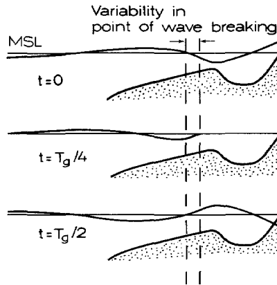
Figure 5.31 Calculated infragravity wave over a barred profile, over one half of the period of the wave groups, T_g . After Symonds and Bowen (1984).
