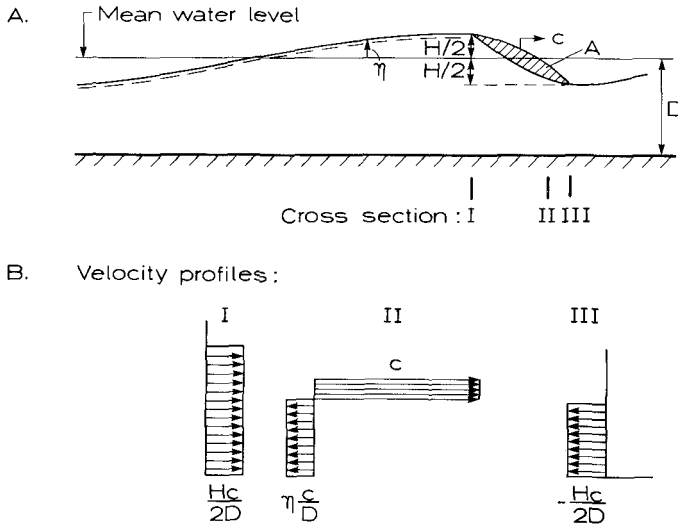
Figure 4.6 A: The structure of a broken wave with a surface roller.
