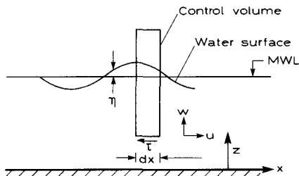
Figure 6.2 Control volume (Eulerian description) to which the momentum equation is applied.
