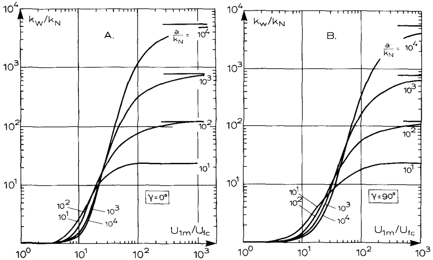
Figure 3.8 Variation of k_w/k_N with U_{1m}/U_{fc} for different values of a/k_N .
