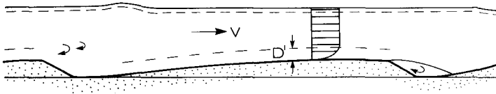
Figure 9.15 Sketch of the boundary layer developed along a dune.
