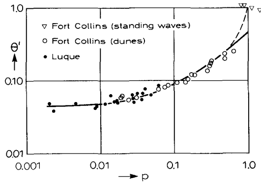
Figure 7.11 Probability p versus non-dimensional effective shear stress \theta' .
