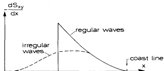
Figure 5.4 Distribution of the longshore driving force, regular waves and irregular waves.
