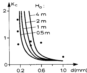
Figure 12.9 Variation in K_c -factor with grain size. Theoretical prediction is based on H_0/L_0 = 0.025 , \beta = 0.01 , and \alpha_0 = 45^\circ . The measured values (filled circles) are from Dean et al. (1982).
