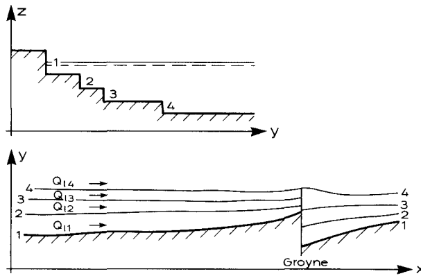
Figure 12.21 The coastal profile and plan form in a multi-line model.
