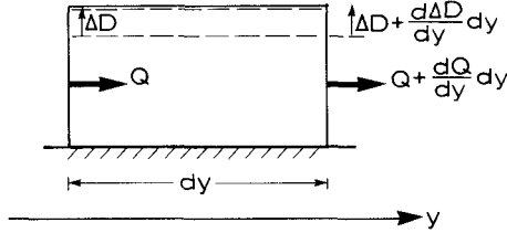
Figure 5.18 Sketch showing the terms in the longshore momentum equation
