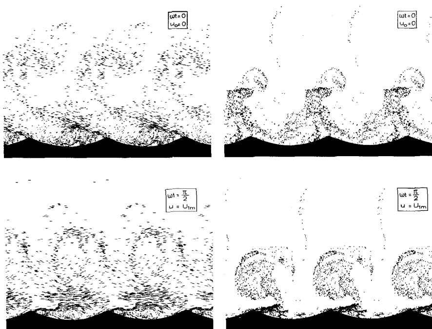
Figure 10.17 Flow pattern (at the left) and suspended sediment particles (at the right) at two phases during a wave cycle. (Hansen et al., 1991).
