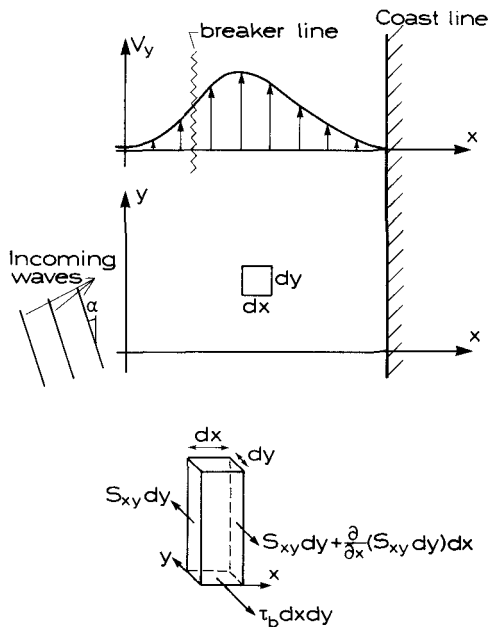
Figure 5.1 Top: The coordinate system and the control volume.
