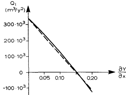
Figure 12.18 The calculated relation between \partial Y/\partial x and Q_l and (dotted line) approximation by a straight line.
