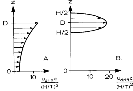
Figure 1.5 Example of the vertical distribution of the drift velocity. A: Calculated by Lagrangian analysis. B: Calculated by Eulerian analysis. D = 10 m, T = 7 sec, H = 4 m.
