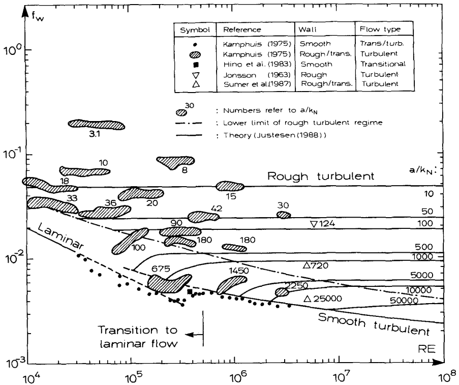
Figure 2.13 Friction factor diagram based on experiments and a one-equation turbulence model. (From Justesen, 1988a).
