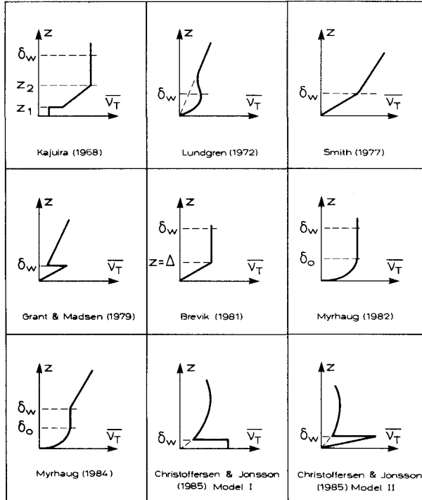
Figure 3.14 Schematic mean eddy viscosity distributions for time-invariant eddy viscosity models. (After Justesen, 1988).
