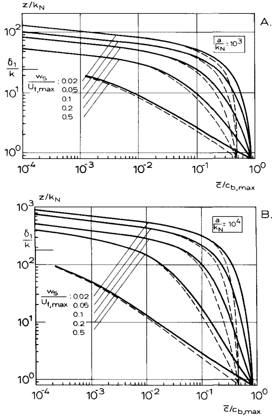
Figure 8.7 Theoretical vertical distribution of the average concentration \bar{c} in pure wave motion. A: a/k_N = 10^3 . B: a/k_N = 10^4 . The fully drawn line corresponds to \theta'_{\max} = 10 , while the dashed line corresponds to \theta'_{\max} = 1 . (Fredsoe et al., 1985).
