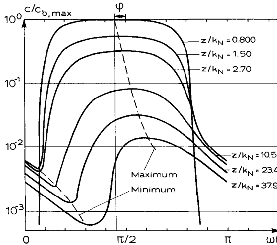
Figure 8.5 Variation in concentration with time at different levels from the bed for a/k_N = 3916 , \theta'_{\max} = 1.45 and w_s/U_{1m} = 0.018 . (Fredsoe et al., 1985).
