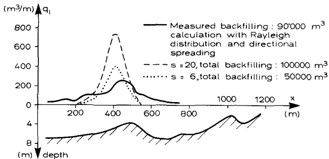
Figure 12.12 Comparison between measured backfilling, cf. Mangor et al. (1984), and calculated backfilling.
