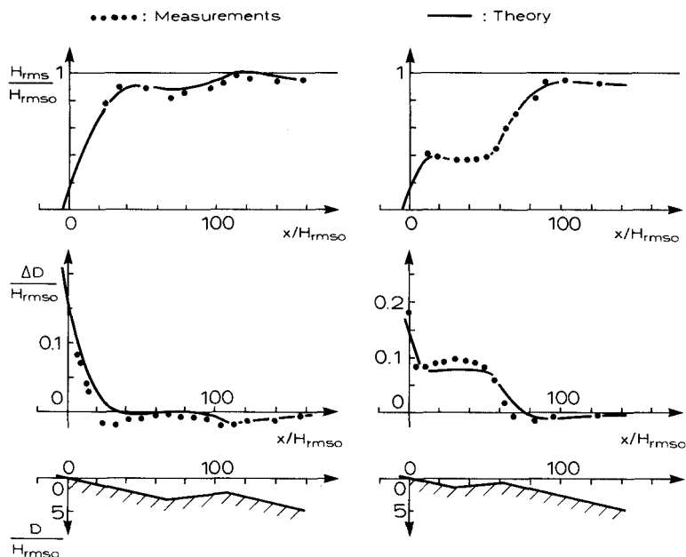
Figure 4.16 Examples of predictions of \Delta D and H_{rms} , after Battjes and Janssen (1978). \cdots : measured data. — : numerical results.
