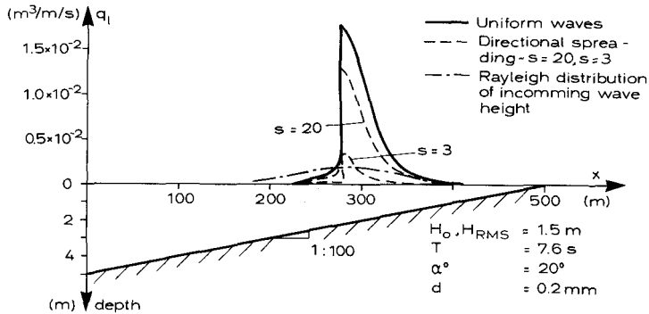
Figure 12.11 Distributions of the longshore sediment transport across a plane coast.
