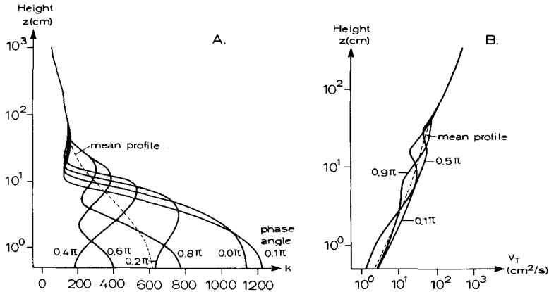
Figure 3.16 Vertical profiles at different phase angles of (A) turbulent kinetic energy and (B) eddy viscosity for the co-linear case. Parameter settings are the same as in Fig. 3.15. The dashed lines indicate the mean distributions. (After Davies et al., 1988).
