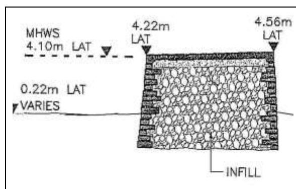
Figure 2.3 Simplified section through Dublin Great South Wall
