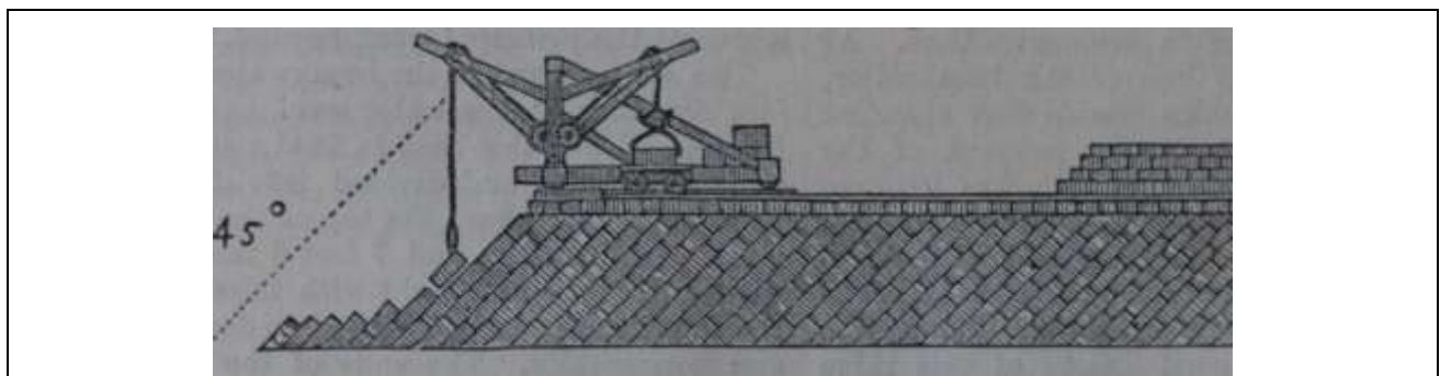
Figure 3.13 Slice blockwork
