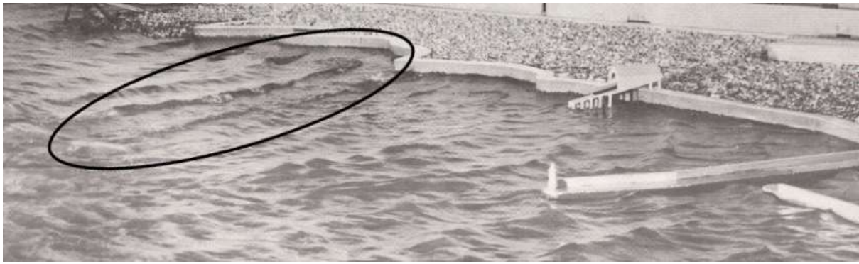
Figure 6.5 Physical model showing enhanced shoaling and breaking at Crane Rocks From HRS (1975), 8s waves
