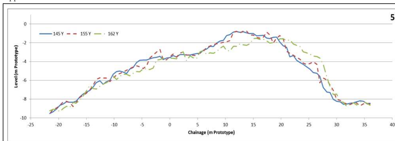
Figure 7.30 Collapsed profiles, Series 5
