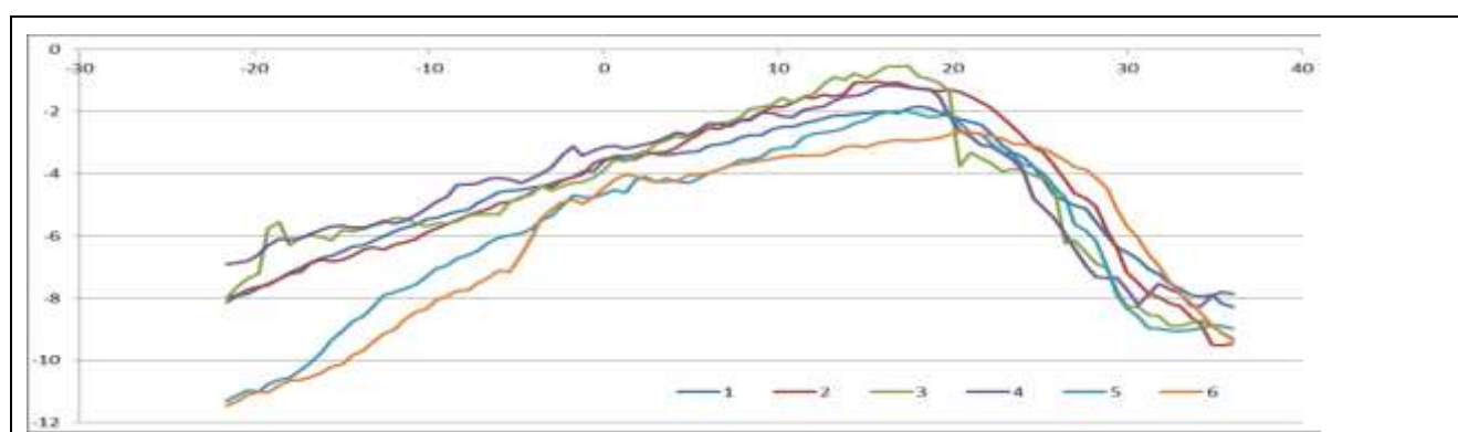
Figure 7.44 Example post-collapse profiles, Series 1-6
