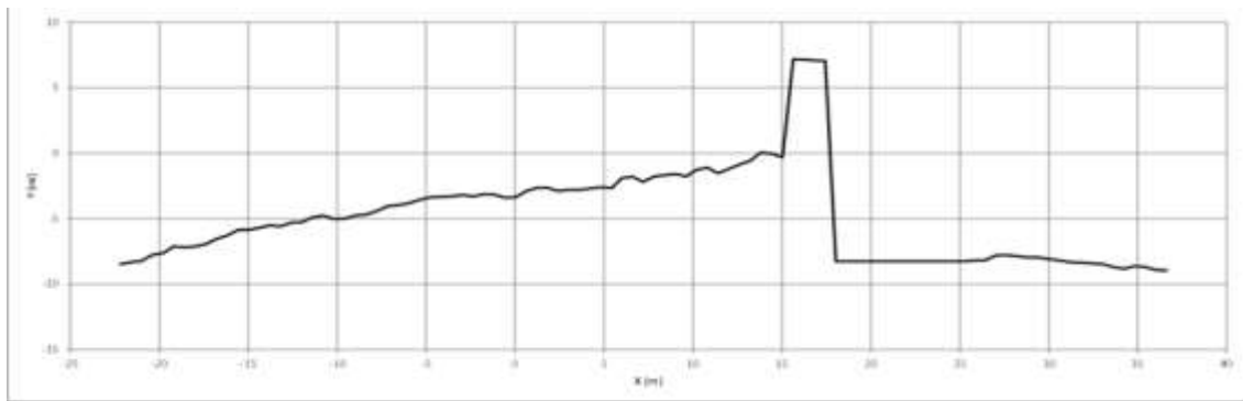
Figure 7.11 Test Series 1, profile taken post seaward wall failure, run 12
