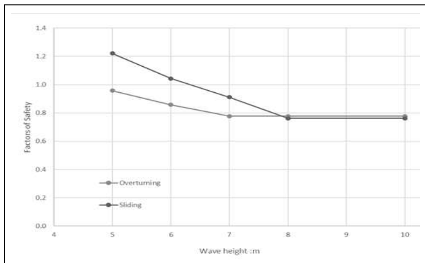
Figure 6.6 Effect of wave height on Factors of Safety
