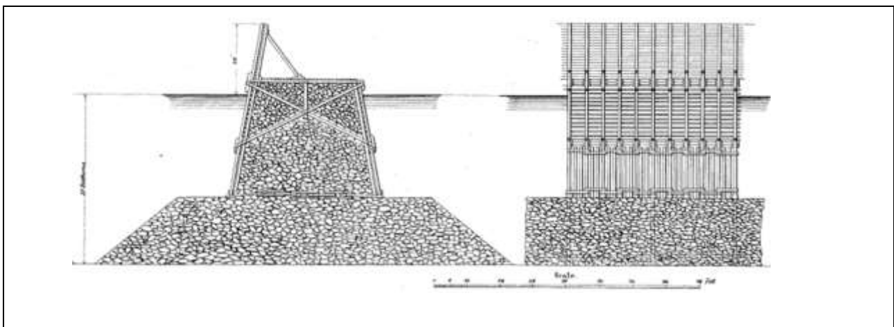
Figure 3.1 Timber crib breakwater After Scott (1858)
