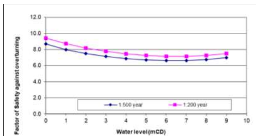
Figure 6.23 Factors of Safety against overturning
