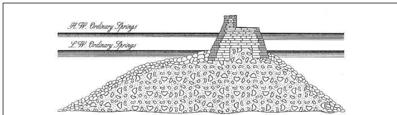
Figure 6.9 Simplified section of outer length of Alderney breakwater mound and wall, showing extended mound
