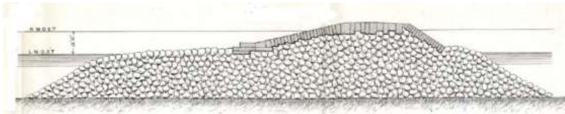
Figure 2.22 Section of Plymouth breakwater
