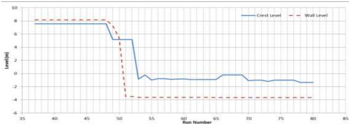
Figure 7.12 Crest height evolution for Test Series 2
