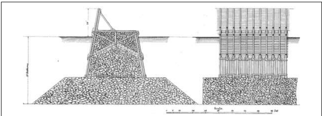
Figure 11.4 Timber crib breakwater
