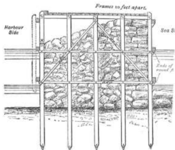
Figure 2.2 Timber-framed breakwater
