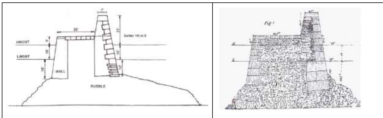
Figure 2.26 Cross-sections of the intended pier After Paxton (2009)
