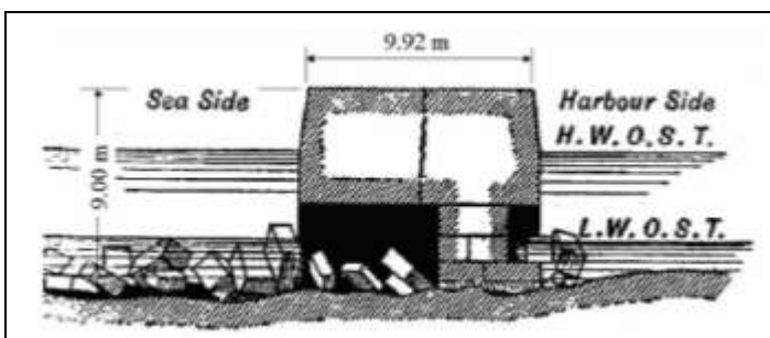
Figure 3.8 Blockwork damage at Aberdeen
