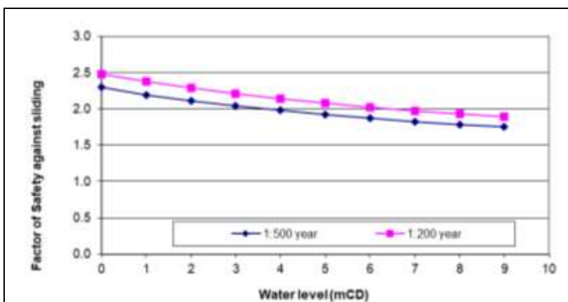
Figure 6.22 Factors of Safety against sliding, \mu = 0.8
