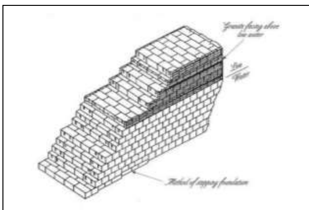
Figure 6.19 Schematic of Dover breakwater blockwork
