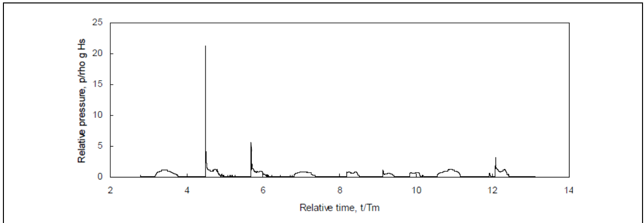
Figure 5.8 Examples of pulsating and impulsive forces
