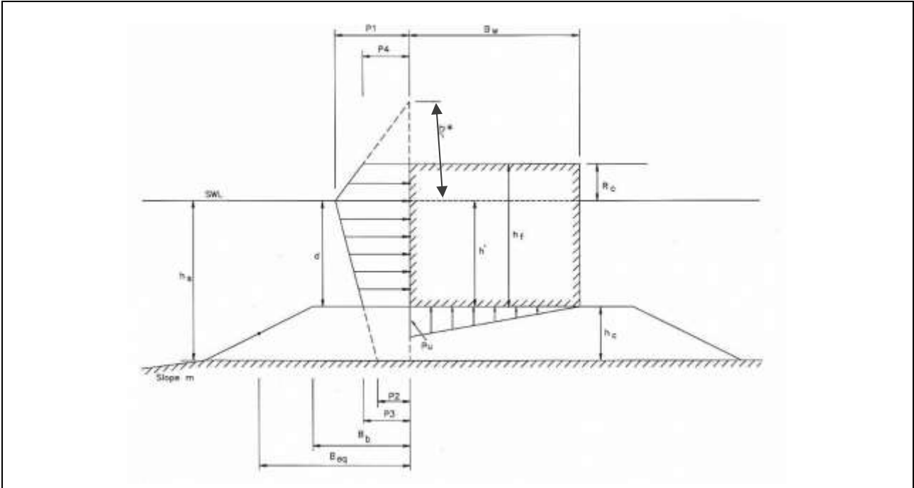
Figure 5.7 Notation used for Goda's equations for wave force
