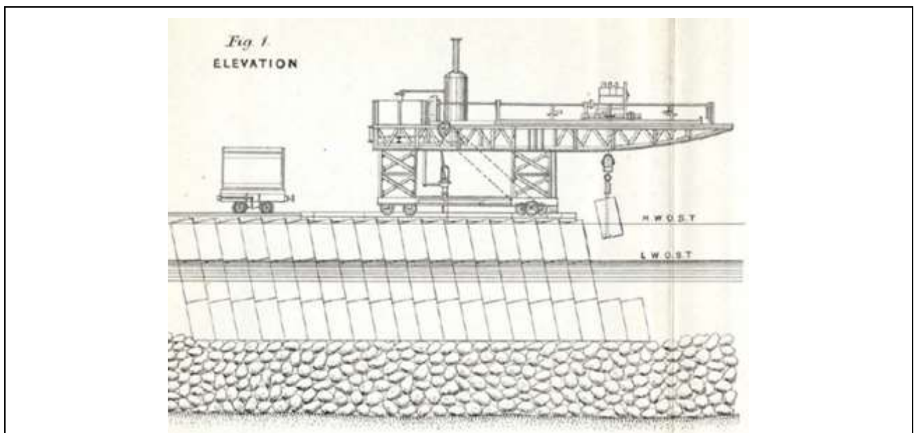
Figure 3.14 Slice blockwork
