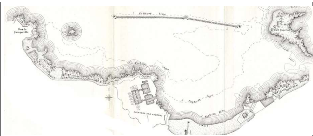
Figure 2.9 Cherbourg harbour
