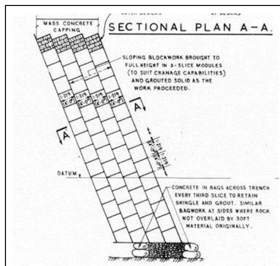
Figure 3.15 Slice blockwork extending the Hermitage Breakwater in 1887-88
