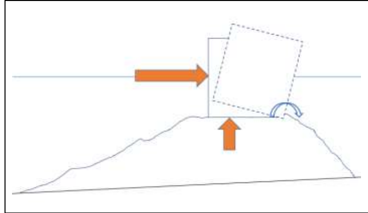
Figure 5.11 Schematic for overturning analysis
