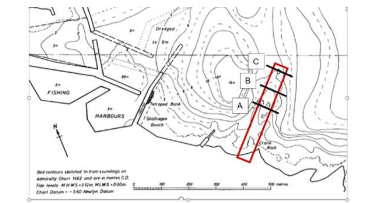
Figure 6.4 Bathymetry of Wick Bay
