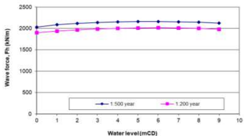
Figure 6.21 Total horizontal wave force, F_h
