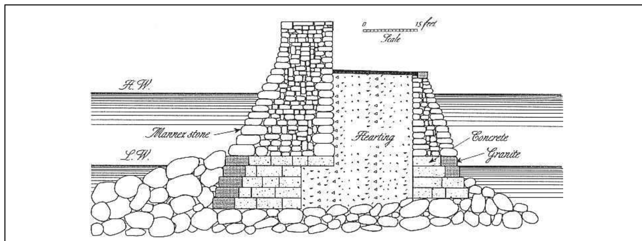
Figure 6.8 Simplified section of Alderney breakwater wall
