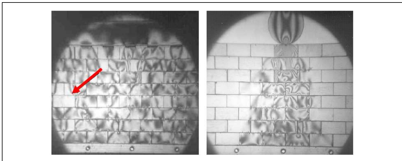
Figure 3.9 Stress paths in photo-elastic material
