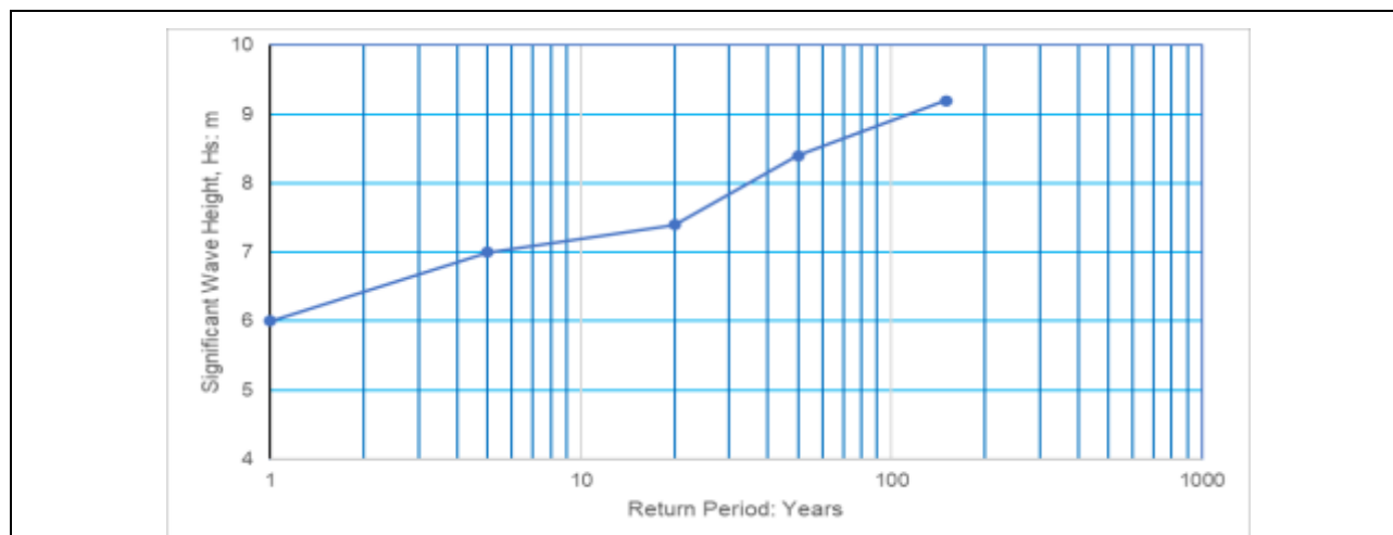
Figure 6.15 Wave conditions from HR Wallingford tests
