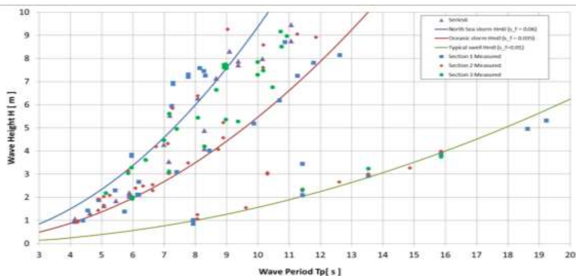
Figure 7.7 Wave conditions for conditions A, B, and C (at 1:30 scale)
