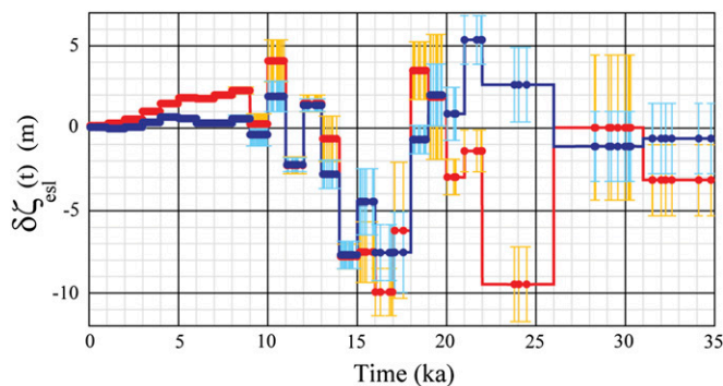
Fig. 3. Low-definition solutions (1,000-y time bins) for the corrective term \delta\zeta^m_{est}(t) for the two lower-mantle viscosity solutions (low-viscosity solution in red with yellow error bars and high-viscosity solution in blue with pale blue error bars).
