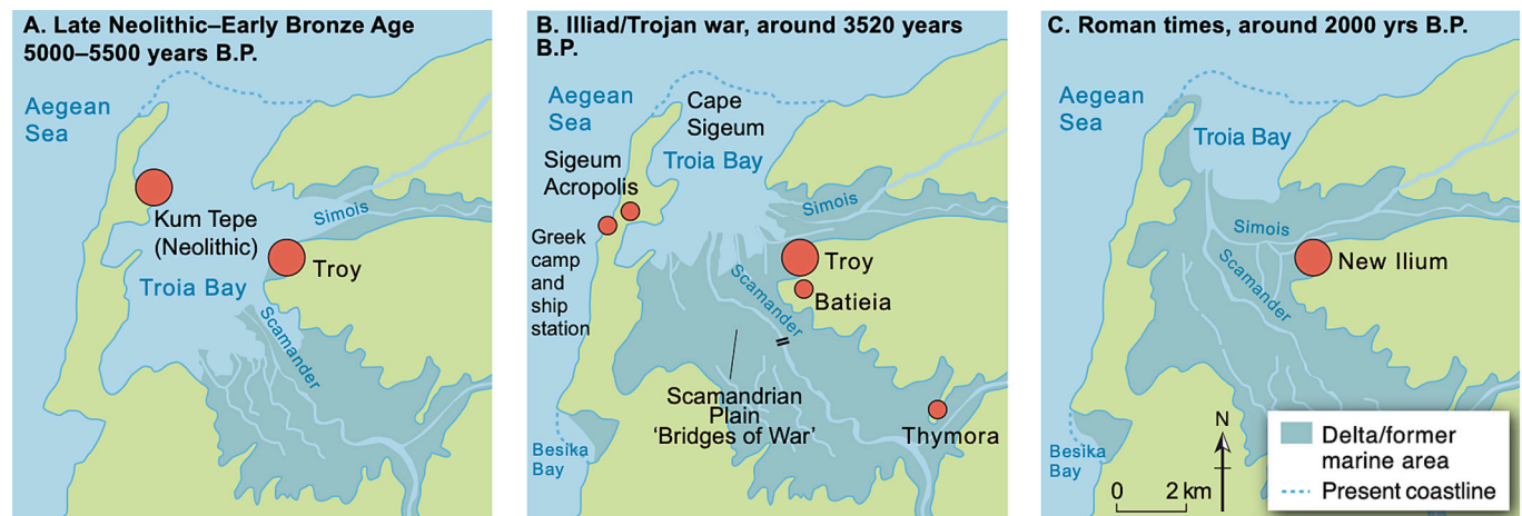
Fig. 8. Delta sedimentation and its effect on ancient human settlements and harbours, with the example of the palaeogeographic evolution of Troia Bay between the Late Neolithic–Early Bronze Age and the Roman period, and the progradation of the Scamander and Simois deltas in Asia Minor (modern Türkiye). Fluvial sediment supply and delta dynamics framed the landscape of ancient Troy. Delta progradation and the seaward-shifting shoreline played a decisive role in its accessibility, harbour potential and long-term settlement history (adapted from Kraft et al., 2003).
