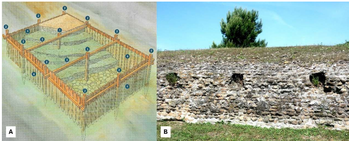
Figure 9. A: Caisson built out from the shore. (Coulon & Golvin, 2020 & Oleson, 2014). B: Portus' north concrete breakwater showing imprints of transverse caisson beams. (Photo de Graauw, 2011)
