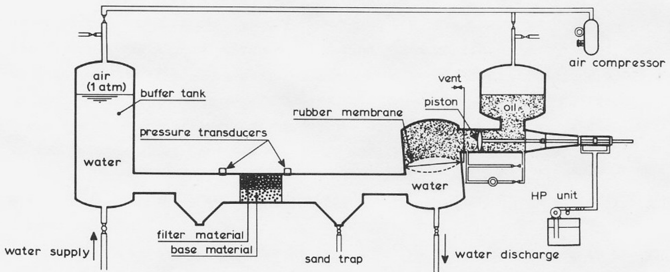
FIG. 4 TEST RIG IN PULSATING WATER TUNNEL
