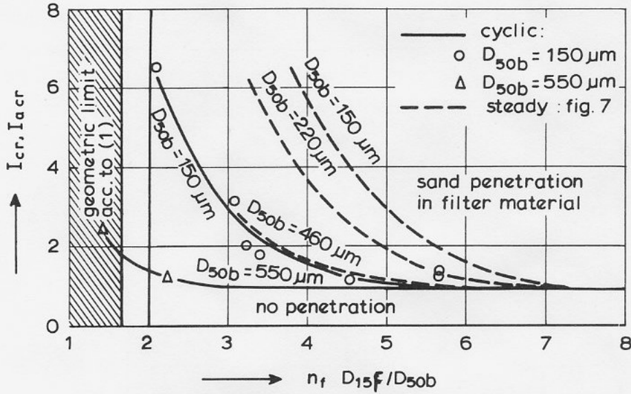
FIG. 9 CRITICAL HYDRAULIC GRADIENTS WITH CYCLIC FLOW PERPENDICULAR TO INTERFACE
