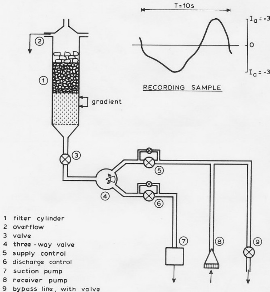
FIG. 8 TEST RIG WITH FILTER CYLINDER
