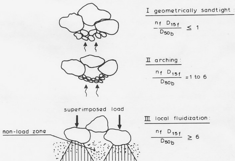
FIG. 12 PHYSICAL EXPLANATION OF FILTER ACTION
