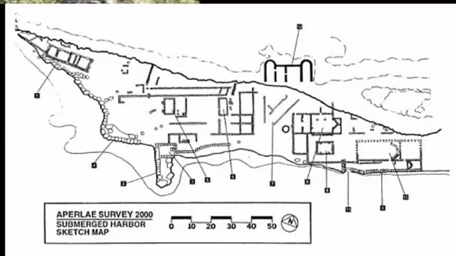
Plan of Submerged Features along waterfront
