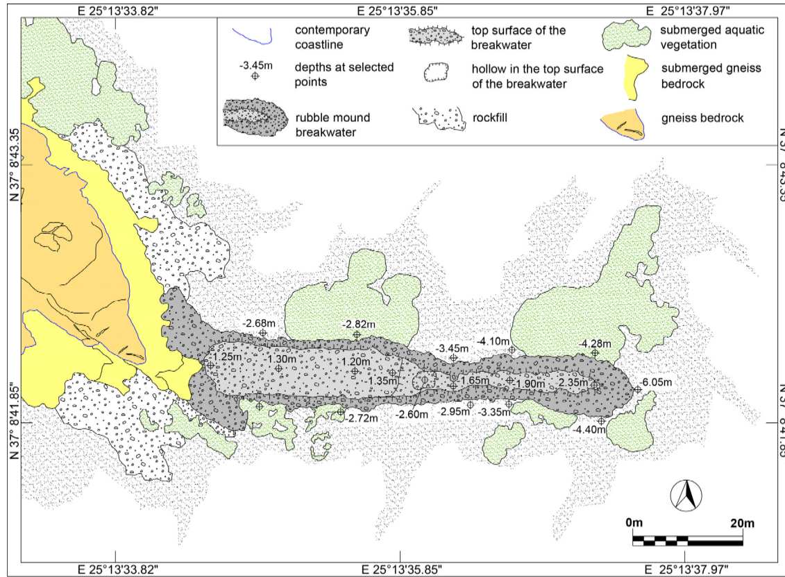
Figure 6. Plan of the rubble mound breakwater of Agios Ioannis Detis.
