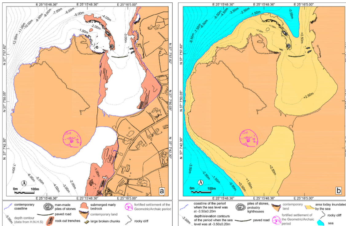
Figure 8. (a) Bathymetric map of Oikonomou Island (depths from H.N.H.S.). (b) Palaeogeographic reconstruction of Oikonomou Island when the sea level was at 3.50 \pm 0.20 m bmsl.
