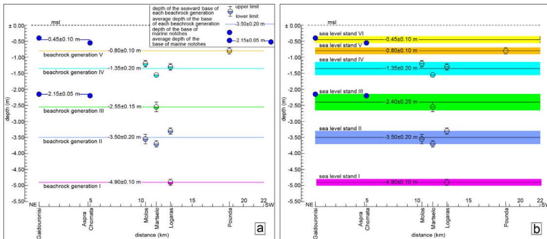
Figure 4. (a) Average depths of the seaward base of each beachrock generation and the base of marine notches identified along the coast of Paros. (b) Sea level stands deduced from the depths of the geomorphological indicators. (msl: mean sea level).
