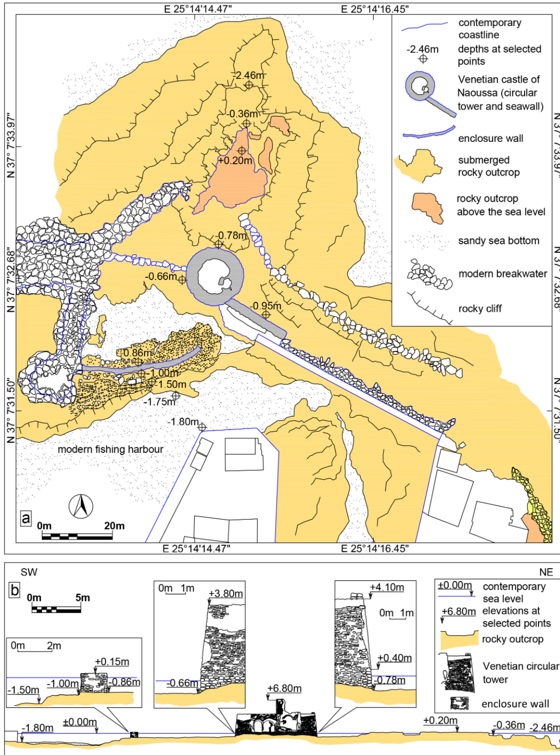
Figure 13. (a) Plan of the Venetian castle of Naoussa. (b) SW-NE cross-section of the castle area.
