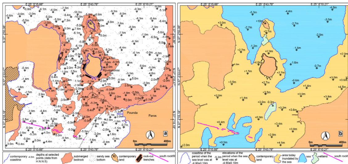
Figure 5. (a) Bathymetric map of the northern section of the Paros-Antiparos Strait (depths from H.N.H.S). (b) Palaeogeographic reconstruction of the northern section of the Paros-Antiparos Strait when the sea level was at 4.90 \pm 0.10 m bmsl.
