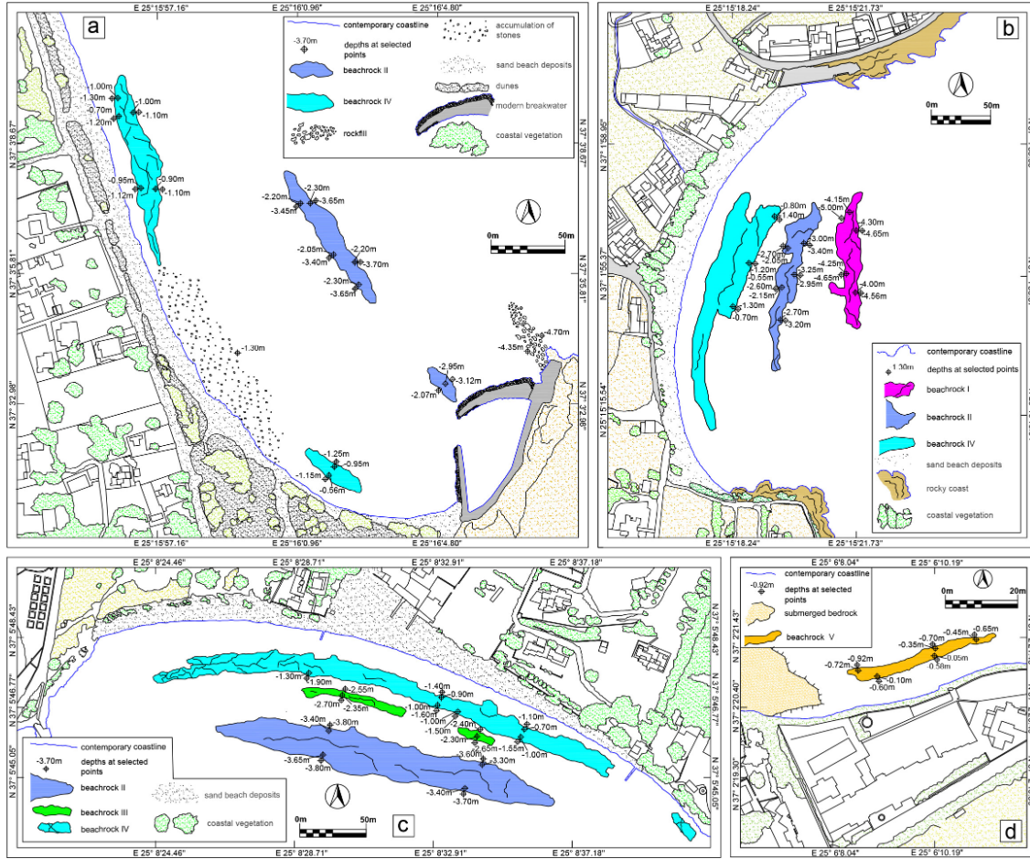
Figure 3. Beachrock generations: (a) Molos Bay, (b) Logaras Bay, (c) Martsele coast, (d) Pouna coast.
