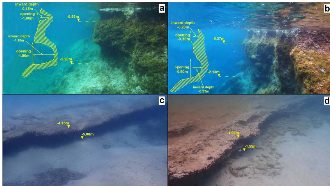
Figure 2. Submerged marine notches on the rocky coast of: (a) Aspra Chomata and (b) Gaidouronisi Islet (NE Paros) GEOSWIM - Paros 2017 project (photo from GEOSWIM - Paros 2017 project). Submerged beachrocks: (c) Logaras Bay (generation I) and (d) Martselo coast (generation IV).
