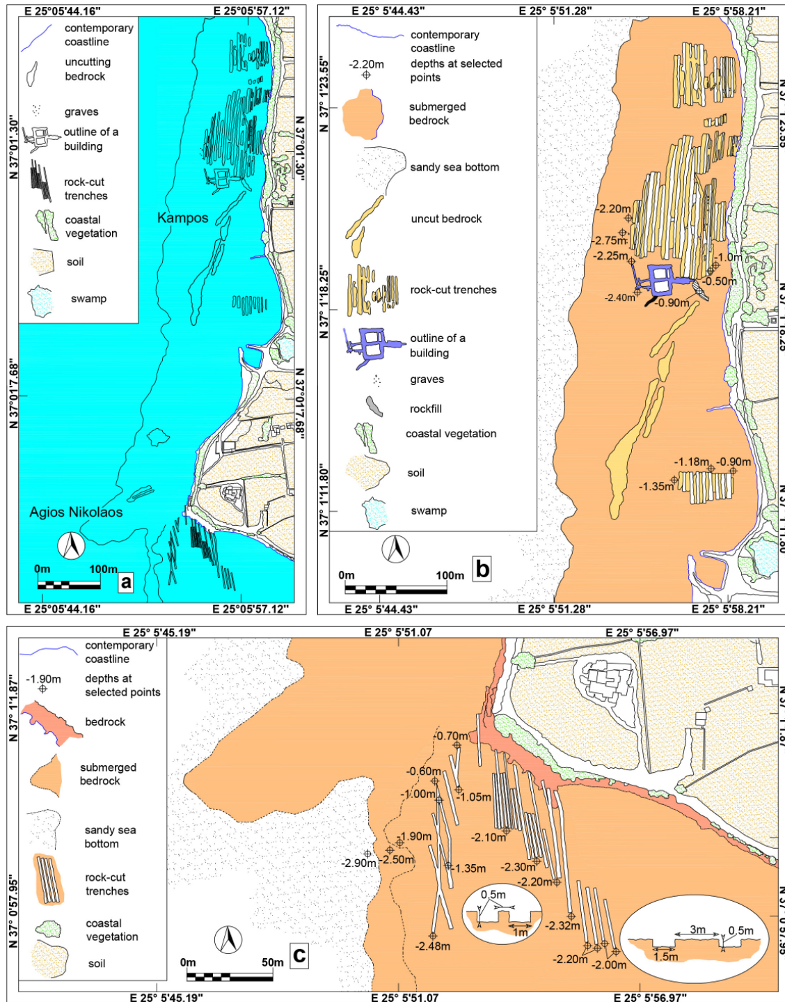
Figure 9. (a) General plan of the submerged rock-cut trenches on the Kampos coast and on the Agios Nikolaos coast (West Paros). (b) Plan of the submerged rock-cut trenches, building and graves on the Kampos coast. (c) Plan of the submerged rock-cut trenches on the Agios Nikolaos coast.
