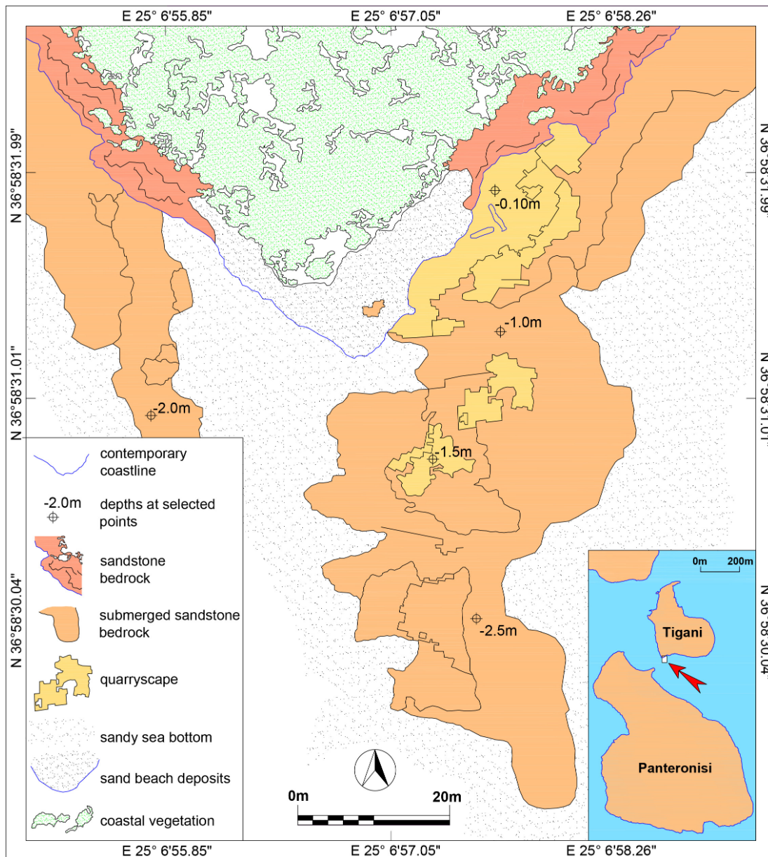
Figure 12. Plan of the submerged quarry on the south coast of Tigani Islet.
