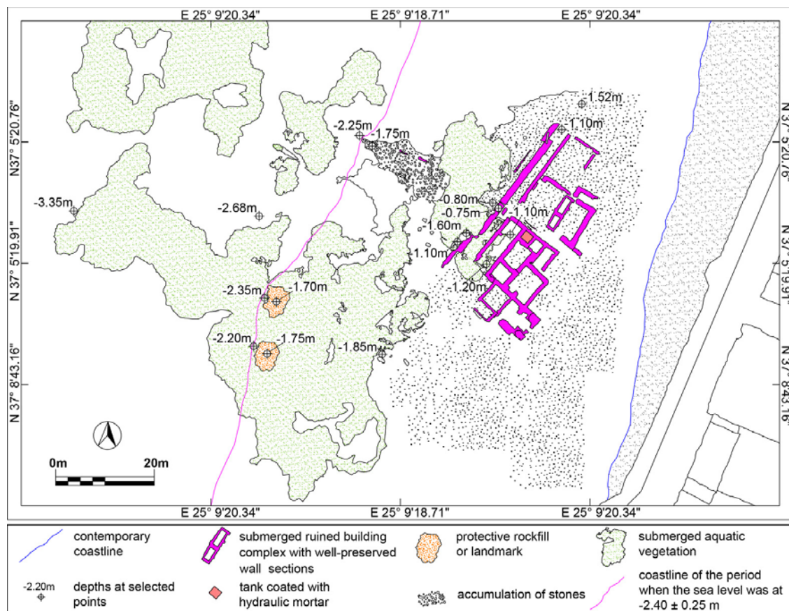
Figure 10. Plan of the submerged building complex in Paroikia Gulf.
