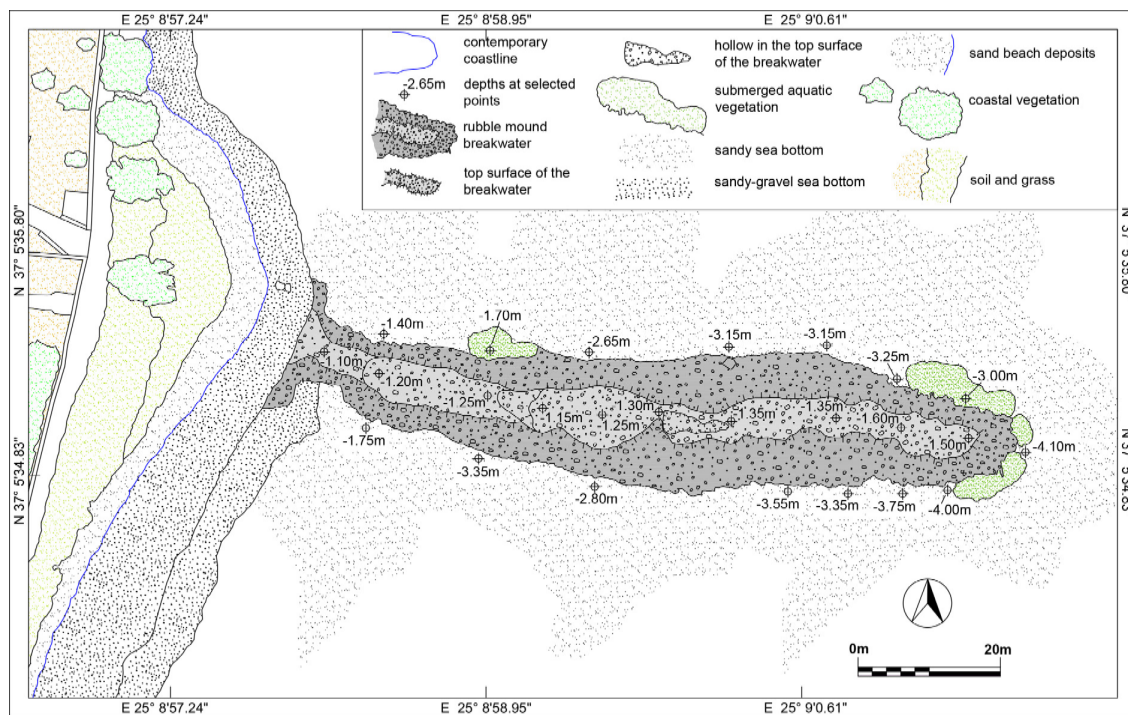
Figure 11. Plan of the rubble mound breakwater of Krotiri in Paroikia Gulf.
