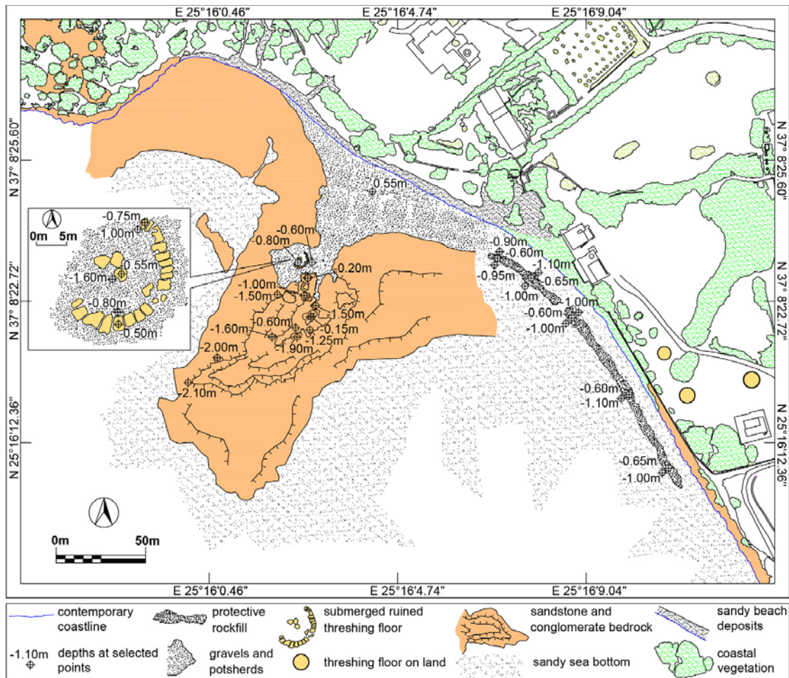
Figure 14. Plan of the Lageri coast.
