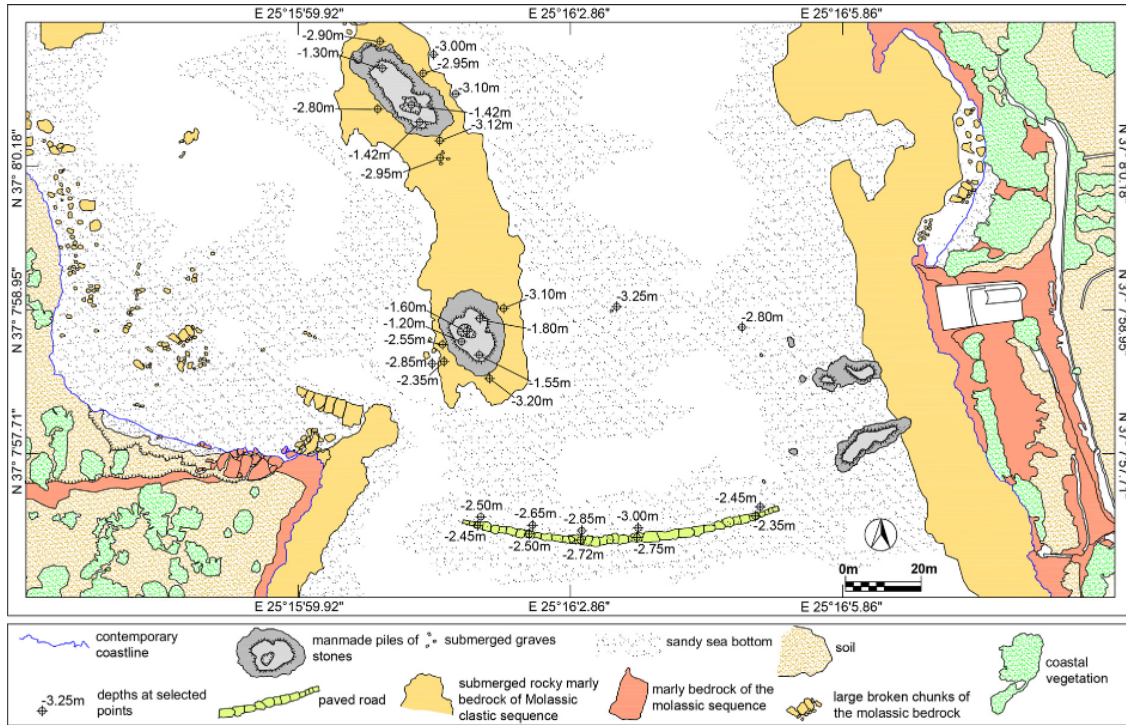
Figure 7. Plan of the northern end of Zoodochos Pigi Bay, in which the submerged structures are indicated.
