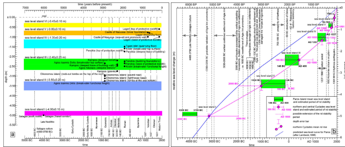
Figure 15. (a) The functional height of the dated archaeological rsl indicators in relation to the six sea level stands determined for Paros Island. (b) The rsl curve for Paros during the last 6,300 years with respect to the rsl curve of the northern and central Cyclades. Important historical and geodynamic events are highlighted. (msl: mean sea level).
