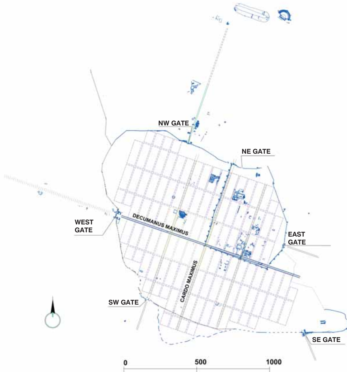
Fig. 124 | Drawing of the urban fabric of Nikopolis. Scientific Committee of Nikopolis (Ch. Tsakoumis and D. Kalpakis).
