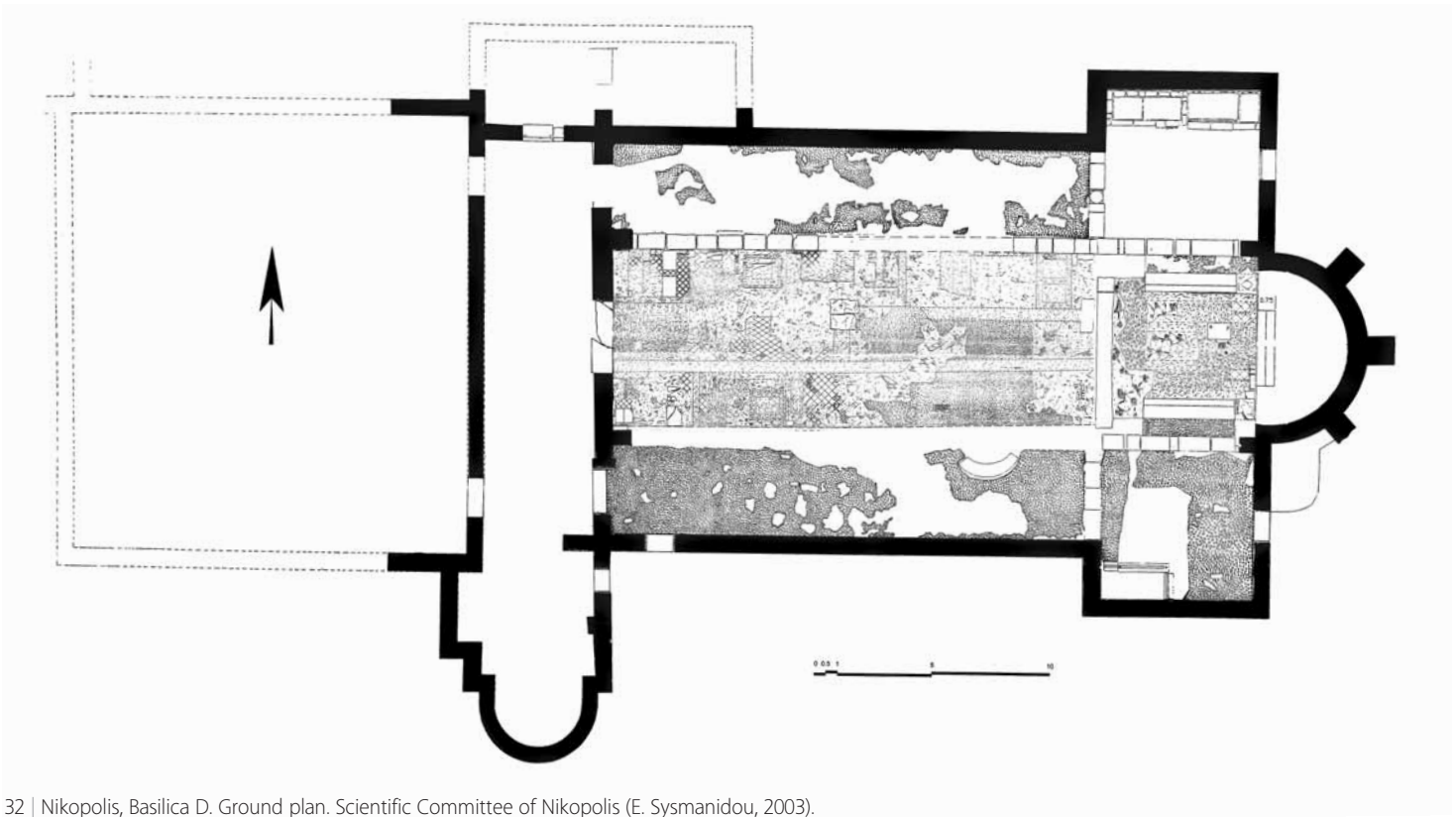
Fig. 132 | Nikopolis, Basilica D. Ground plan. Scientific Committee of Nikopolis (E. Sysmanidou, 2003).
