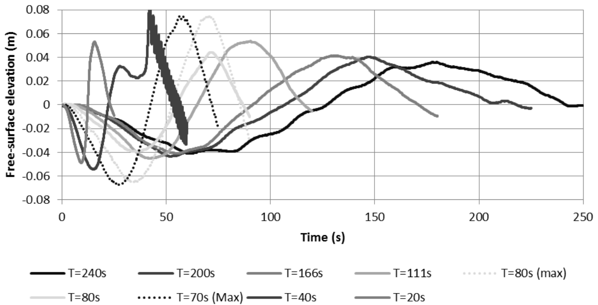
Figure 7 Calibrated N-waves using 2 nd generation TS, measured at the toe of the bathymetry (WG_05).
