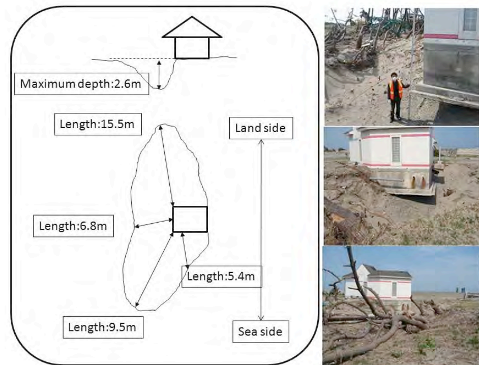
Figure 1 - Scour pattern and multiple views of reinforced concrete structure: Arahama Beach, Sendai, Japan, May 16, 2011, two months after tsunami.
