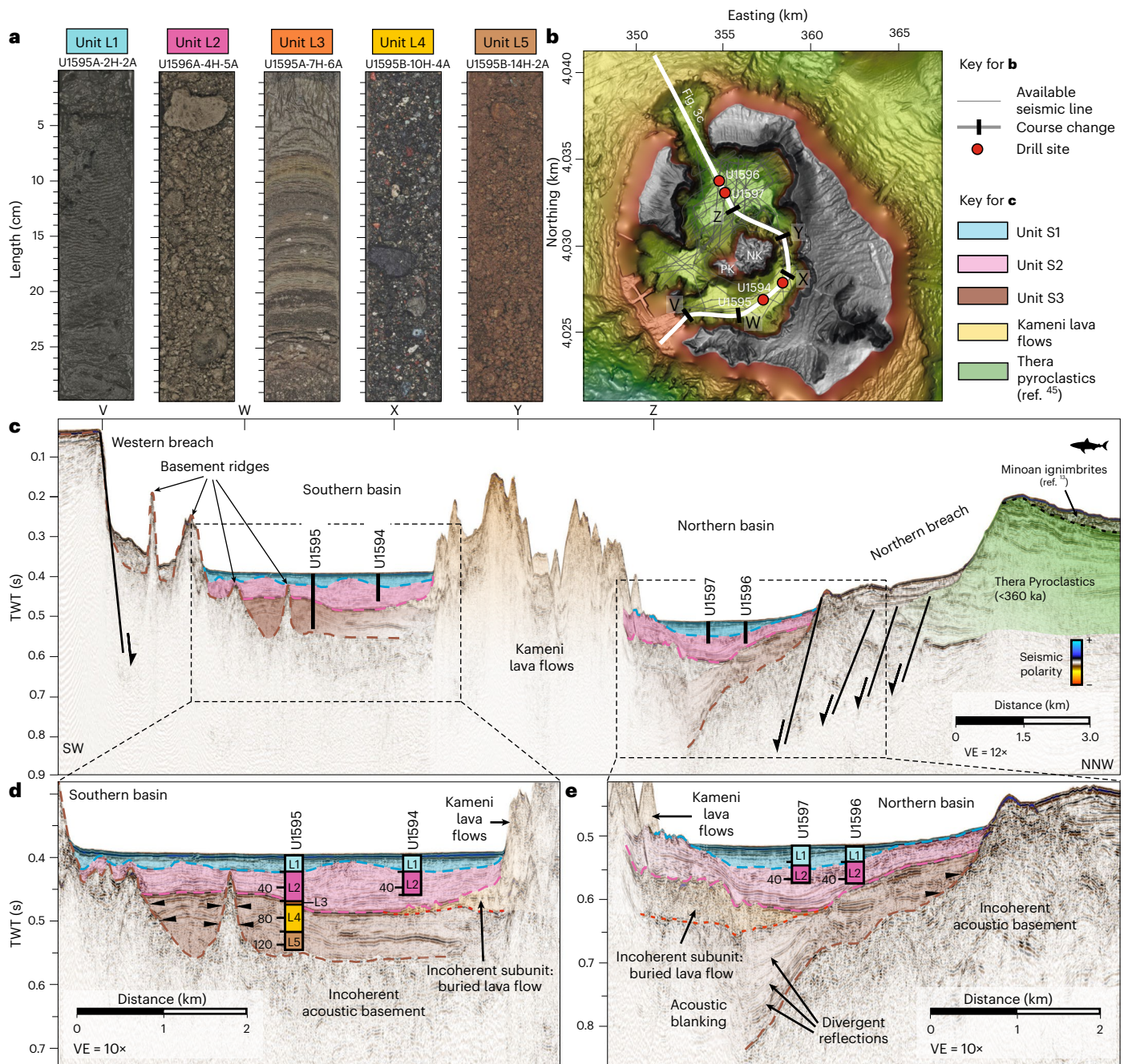
Fig. 3 Core–seismic integration of the intra-caldera sites. a , Representative photos of the five lithologic units L1–L5. b , Overview map with all available seismic profiles in the caldera (grey) and the location of the seismic profile shown in c . The labelled black markers (V–Z) indicate course changes of the seismic profile. c , Seismic profile crossing the Santorini caldera from the western breach across the southern and northern basins towards the northern breach 13,45 . Labelled black lines (V–Z) mark the course changes of the seismic profile. For location, see b . TWT, two-way travel time; VE, vertical exaggeration.
