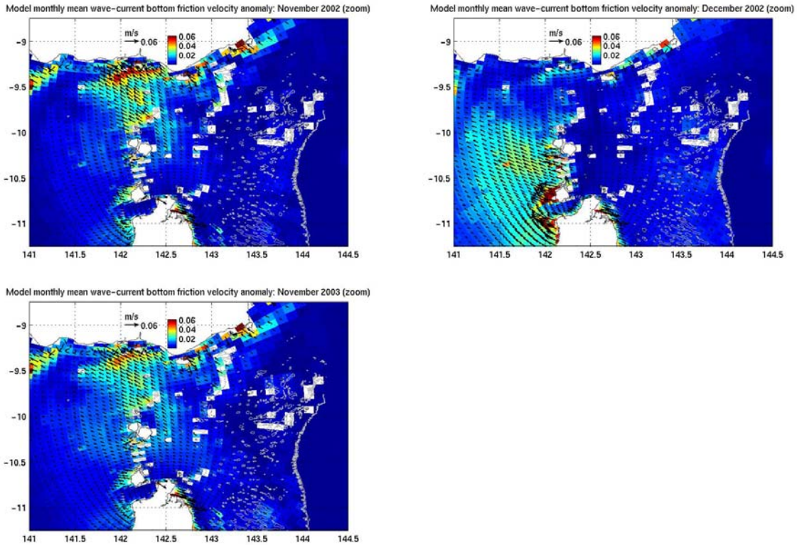
Figure 60: Wave-current bottom friction velocity anomaly indicating a sustained northwestward trend over November and December 2002 and November 2003. Detailed monthly mean anomalies are presented in Appendix 9.5 .
