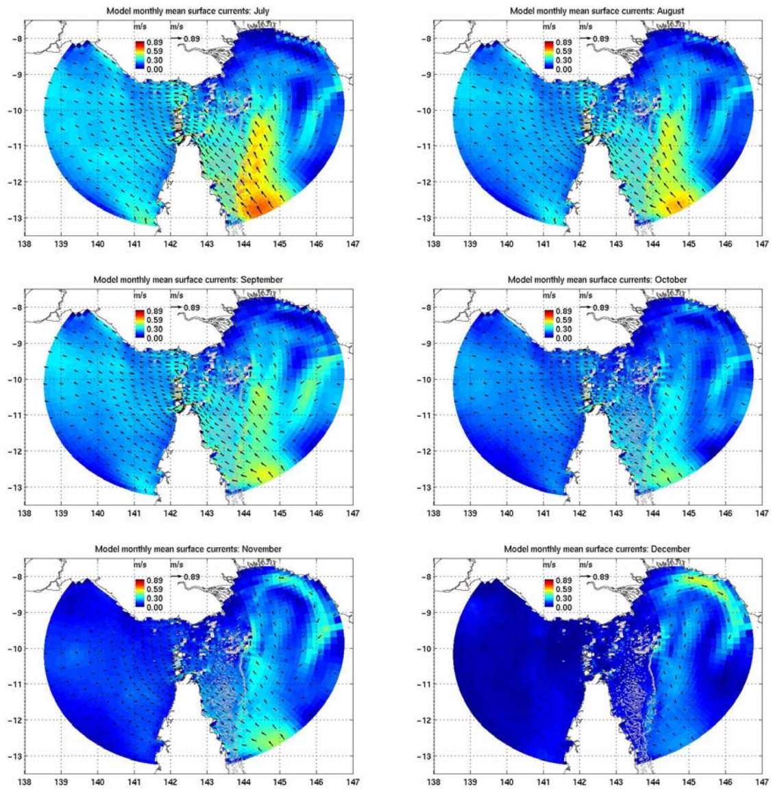
Figure 45: Monthly mean surface currents based on eight years of model runs covering the period 1997-2004 (July to December).
