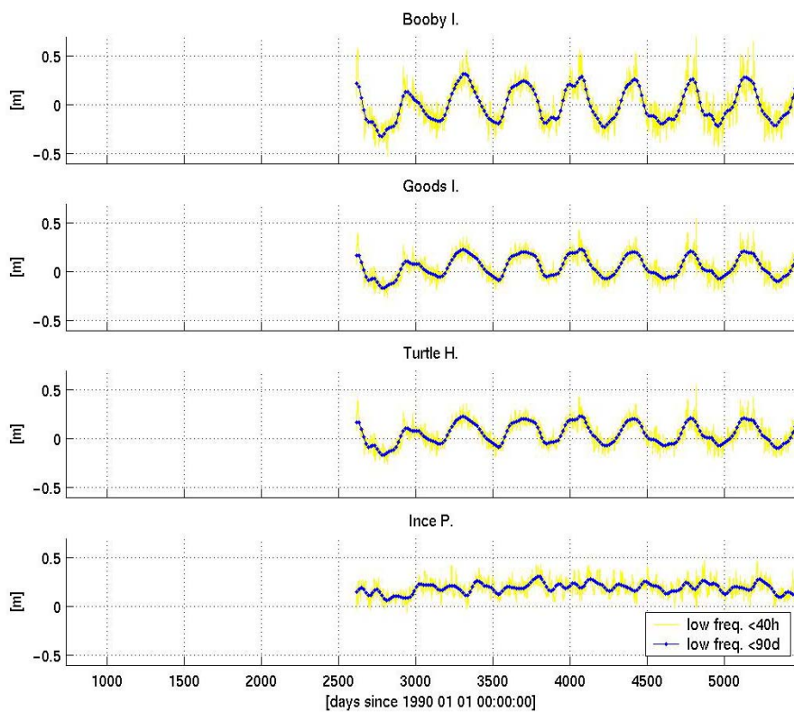
Figure 24: Low pass filtered model sea level time series using a cut off period of 40 hours (yellow) and 90 days (blue).
