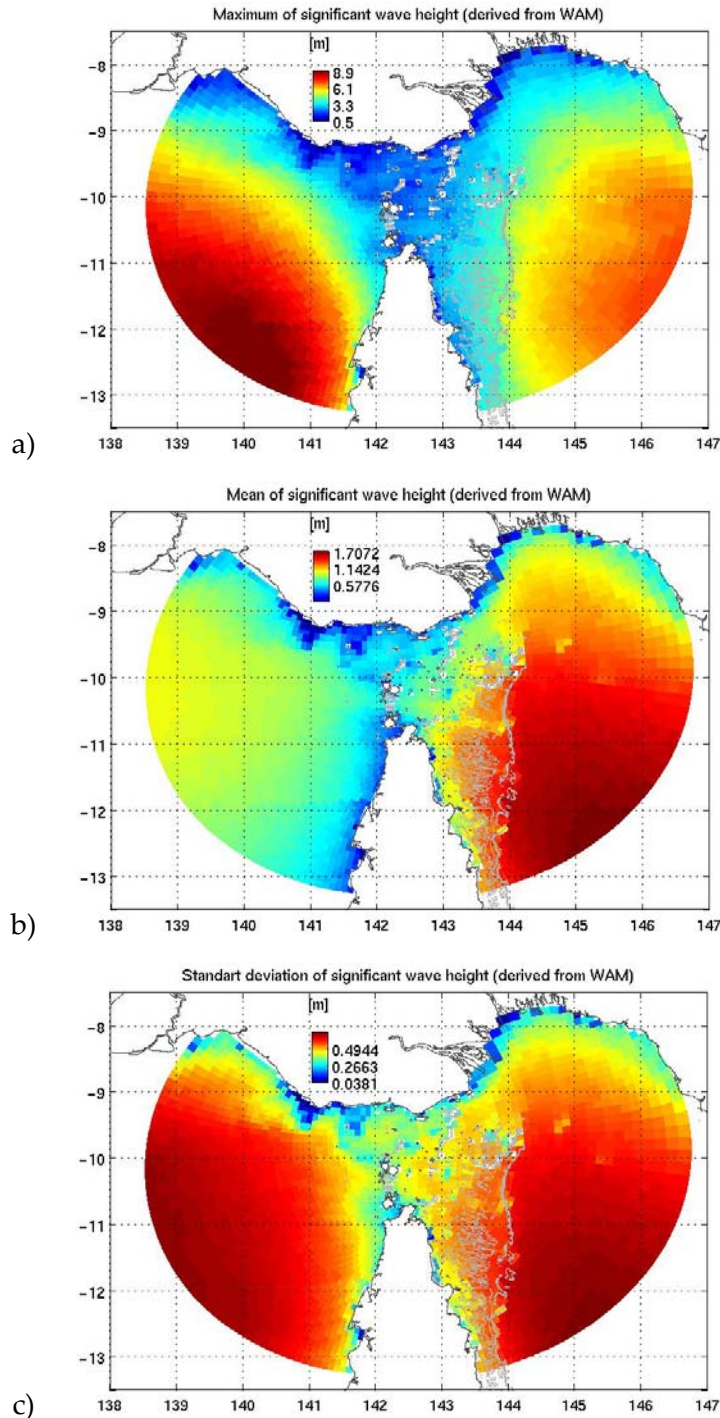
Figure 10: Significant wave height statistics on the hydrodynamic model grid: a) maximum; b) mean; and c) standard deviation. These statistics were derived from WAM outputs covering the period 01/03/1997 to 28/02/2002. Maximum wave heights of up to 9 m in the Gulf of Carpentaria were in response to a tropical depression that developed northeast of Darwin in late December 1997. In other areas of open water maximum wave heights were more typically around 7m, while in the shallow waters of Torres Strait and neighbouring coastal areas they did not exceeded 3m. Mean wave heights in northwest Torres Strait and Gulf of Papua were less than 0.6 m, increasing to around 1.0 m in the southeastern part of the Strait and Gulf of Carpentaria, and 1.5 m in the Coral Sea. While variability (as measured by the standard deviation) followed similar patterns to the mean, its magnitude in the Gulf of Carpentaria was similar to that in the Coral Sea.
