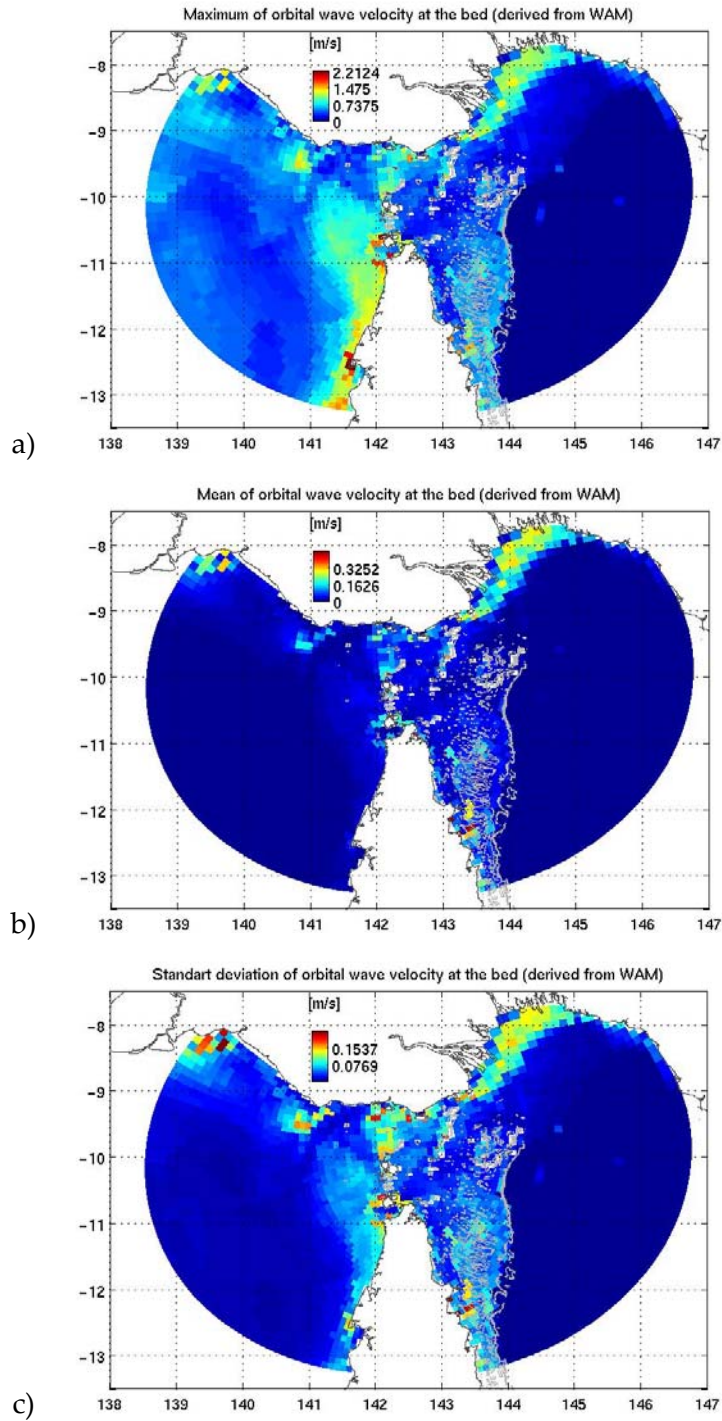
Figure 13: Wave orbital velocity statistics at the seabed: a) maximum; b) mean; and c) standard deviation. Statistics were derived from WAM outputs covering the period 01/03/1997 to 28/02/2002.
