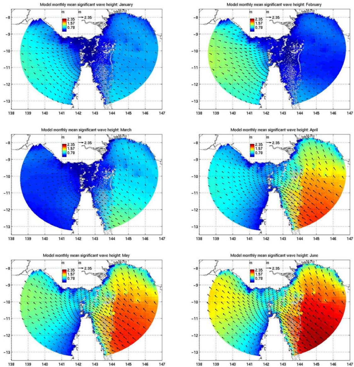
Figure 8: Monthly mean significant wave height and direction (January to June). These fields were calculated by vector averaging the 6 hourly outputs of the BOM-WAM dataset across the years 1997 to 2005. They show that wave direction followed wind direction. Wave heights peaked during the Trades and were significantly higher in the Coral Sea than in the Gulf of Carpentaria.
