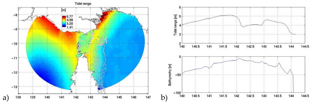
Figure 39: (a) Model tidal range and (b) tidal range profile (top) and corresponding bathymetry (bottom) along 10°S.
