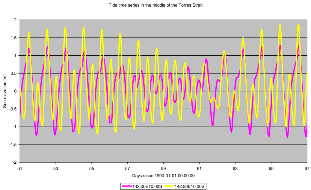
Figure 37: Poorly correlated ( r_2=0.13 , s=0.42 ) tidal signals on the middle of the Torres Strait between the two locations: 142.00E 10S and 142.50E 10S.
