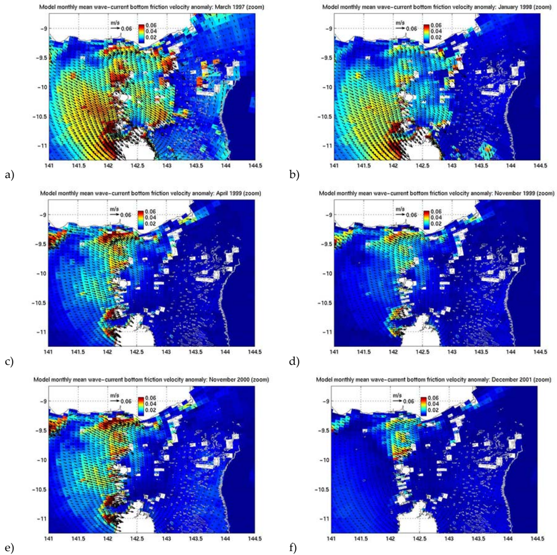
Figure 58: Wave-current bottom friction velocity anomaly indicating persistence of the monsoon through March 1997 and April 1999 and an enhanced monsoon in January 1998 (a, b and c). November 1999 and 2000 show an early monsoon and southeastward trend, while December 2001 shows another enhanced monsoon (d, e and f). Detailed monthly mean anomalies are presented in Appendix 9.5 .
