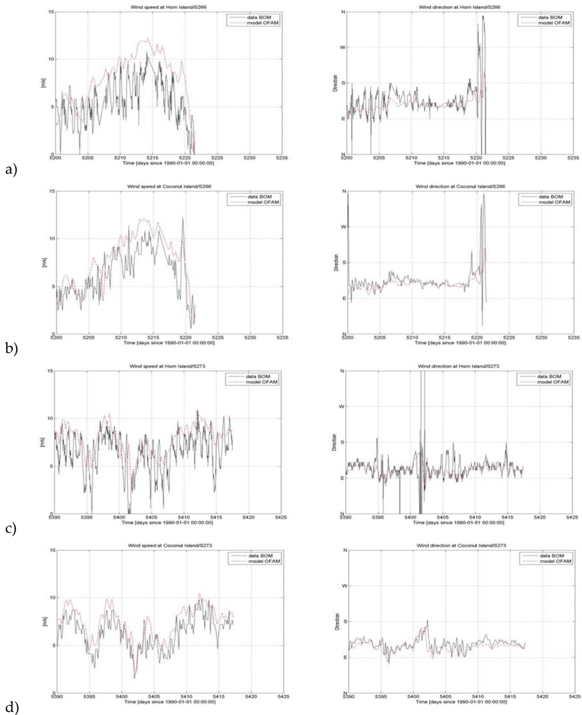
Figure 5: Time-series of wind speed (left) and direction (right) comparing the interpolated OFAM winds (from ECMWF) and locally observed winds (Bureau of Meteorology) for surveys S266 (a, b) and S273 (c, d) at Horn Island [10.48S; 142.29E] and Coconut Island [10.05S; 143.07E]. Modelled winds are in good agreement with maximum daily winds speed. Sub diurnal frequencies including sea breezes are not captured by the global wind model. The main wind cardinal direction is respected.
