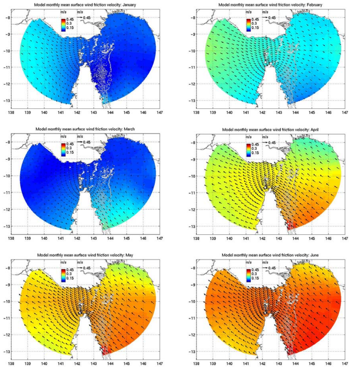
Figure 3: Monthly mean surface wind friction velocity (January to June). These fields were calculated by vector averaging the 6 hourly outputs of the ECMWF dataset across the years 1997 to 2005. They show the prevailing cycle of southeasterly trade winds over winter, switching to northwesterlies over summer as the trades are displaced to the south by equatorial westerlies. Surface wind stress is given by the product of air density ( 1.2 \text{ kg m}^{-3} ) and the square of surface wind friction velocity.
