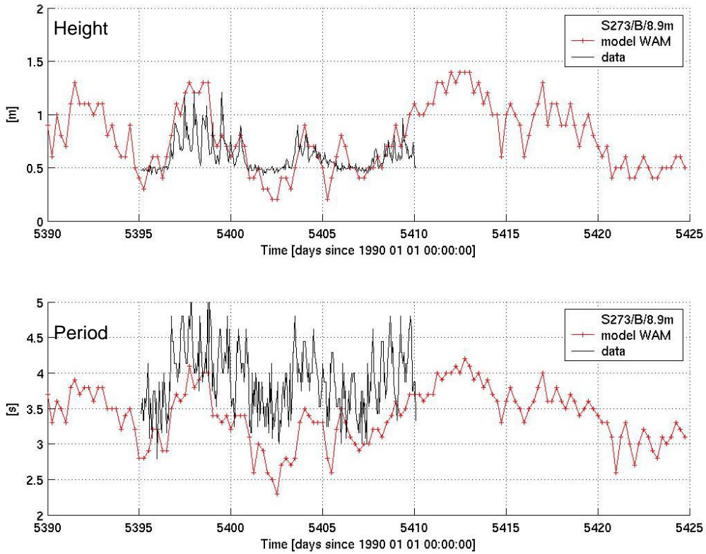
Figure 11: Time-series comparisons between the interpolated WAM data and locally observed waves characteristics, including significant wave height and period for survey 273. The direction of waves has not been measured on the field.
