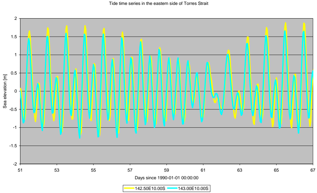
Figure 36: Well-correlated ( r_2=0.82 , s=0.83 ) tidal signals on the eastern side of the Torres Strait between the two locations: 142.50E 10S and 143.00E 10S.
