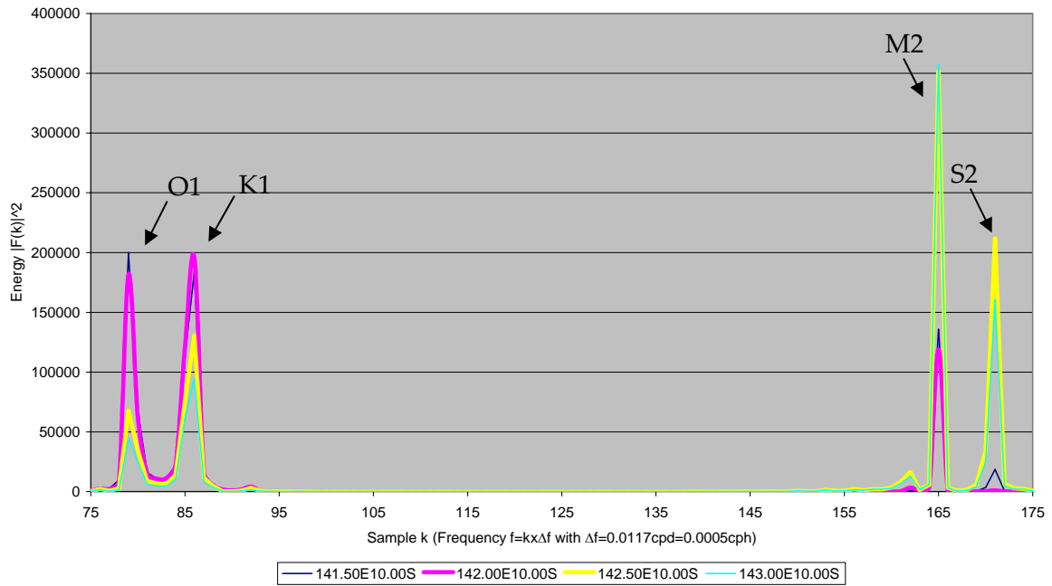
Figure 38: Power spectral density of sea level along the Torres Strait; 90% of the tidal energy is within this range of frequencies.
