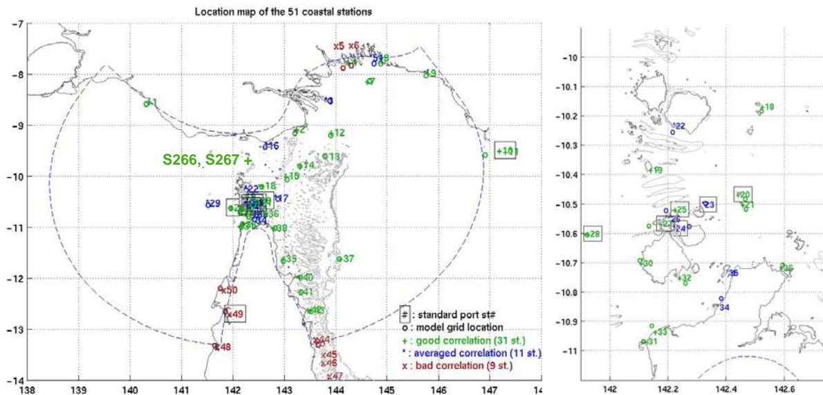
Figure 16: Location of tidal stations, including Admiralty coastal ports and recent survey moorings, used to validate model sealevel estimates. The quality of correlation with observed sealevel is represented by: (+) good quality corresponds to |s-1| < 0.2 and |r2-1| < 0.2 , (x) poor quality correspond to |s-1| > 0.4 & |r2-1| > 0.4 and (*) averaged quality otherwise
