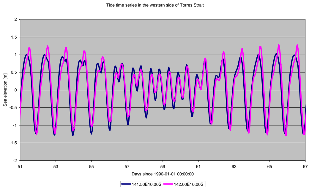
Figure 35: Strongly correlated ( r^2=0.86 , s=0.90 ) tidal signals on the western side of the Torres Strait between 141.50E 10S and 142.00E 10S.
