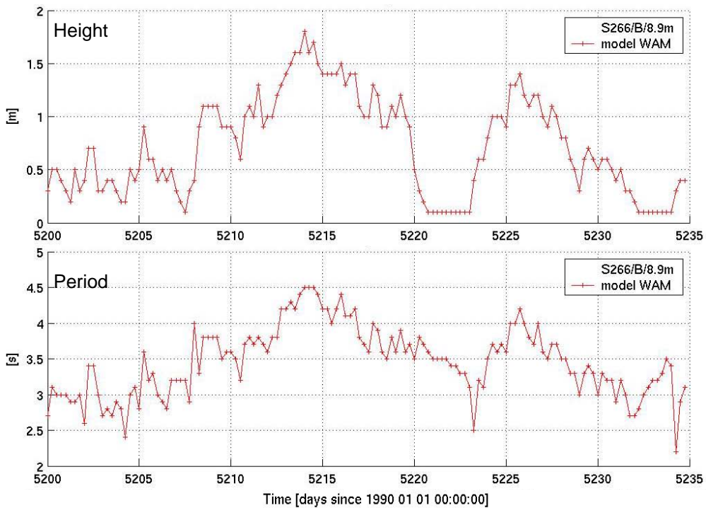
Figure 12: Waves characteristics over survey S266 period derived from WAM. No field data was available from survey S266 due to malfunction of the wave data recorder.
