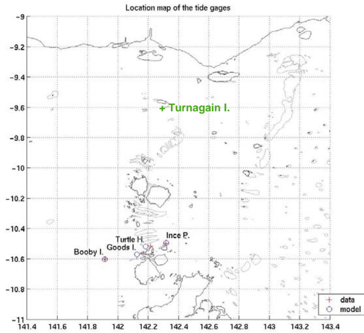
Figure 17: Location map of the four standard port tide gages in Torres Strait, where long term sealevel time series were available. Only short term sealevel time series were available at Turnagain Island.
