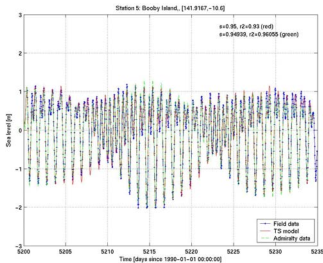
Figure 21: Sea level comparison at Booby Island. Model output from test O and reconstructed sea level from the Admiralty harmonic database are both in very good agreement with field data from the NTC tide gage.
