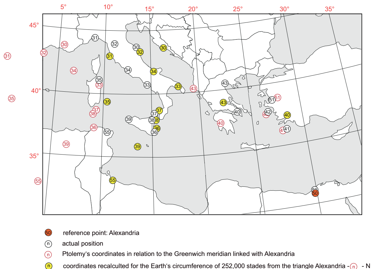
Figure 6: Recalculation of some prominent locations in the eastern Mediterranean for the circumference of the Earth equal to 252,000 stades. The reference point for this recalculation is Alexandria.
