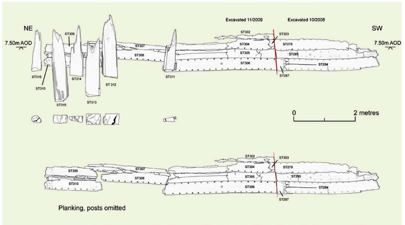
Figure 4 Timbers from a mid 10th-century vessel re-used in a building's wall at Hungate, York.
