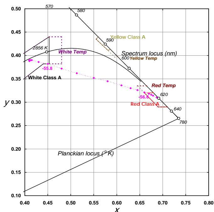
Figure 32 As Figure 31 but plotted on a partial CIE 1931 Chromaticity Diagram
