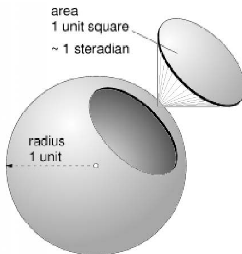
Figure 1 Solid Angle Geometry
