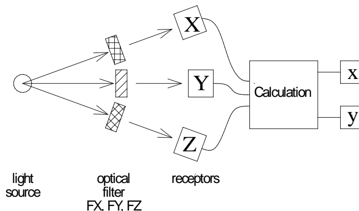
Figure 11 Tristimulus Principle
