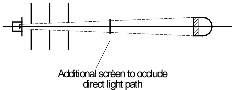
Figure 24 Arrangement to determine ambient and stray light
