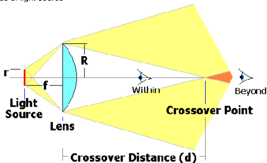
Figure 25 Crossover Distance
