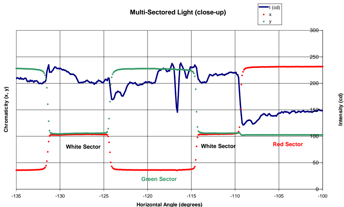
Figure 35 Partial Plot of Sector Light shown in Figure 34 Plotted at 0.1^\circ Intervals
