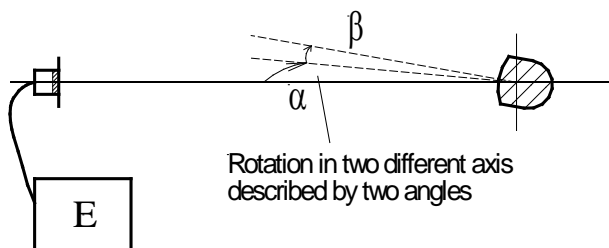
Figure 6 Measurement of Angular Distribution of Luminous Intensity
