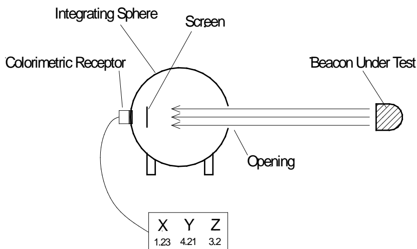
Figure 42 Beacon outside sphere
