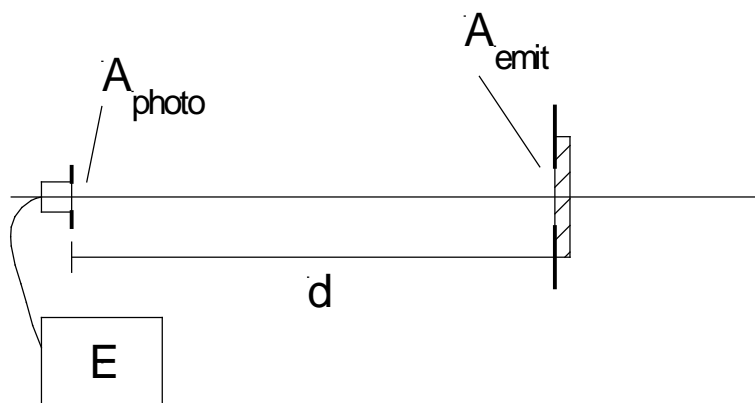
Figure 18 Measurement of Luminance
