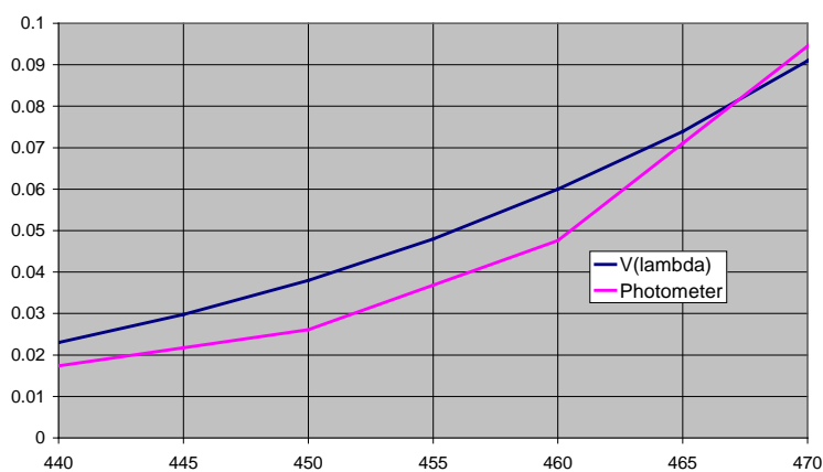
Figure 4 Expanded Section of Spectrum Highlighting Photometric Error in figure 3
