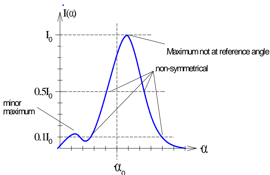
Figure 28 Asymmetrical Intensity Distribution
