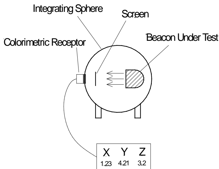
Figure 43 Beacon inside sphere
