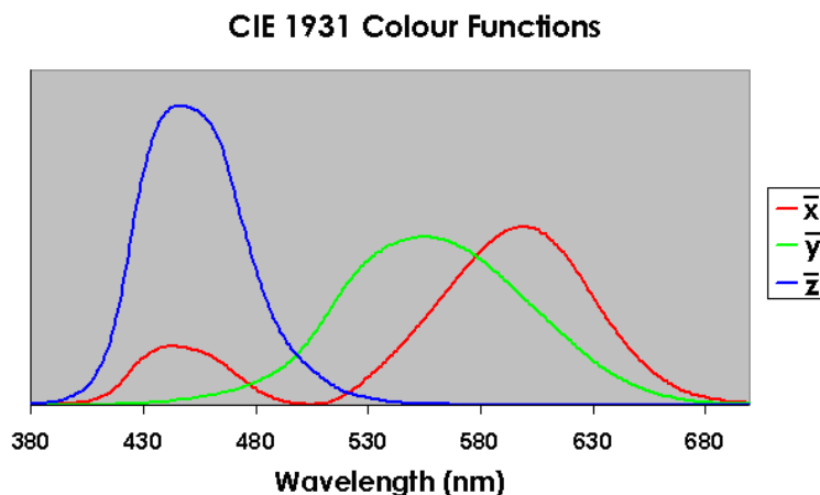
Figure 15 The CIE 1931 Standard Colour Observer
