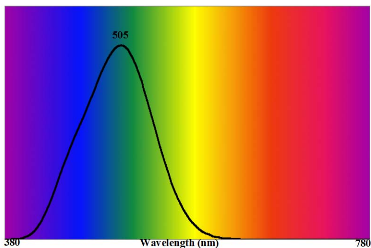
Figure 14 Scotopic Luminous Efficiency Function V'(\lambda)
