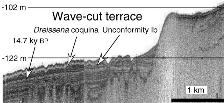
Figure 17 A wave-cut terrace at -120 m on the Ukraine margin associated with the earlier regression that produced unconformity 1b.
