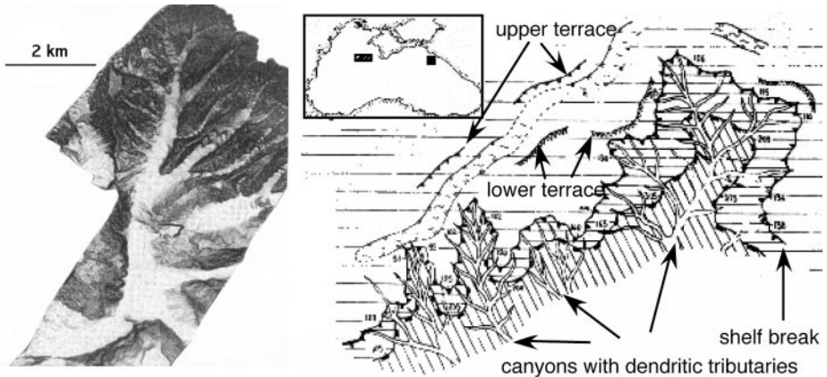
Figure 10 Dendritic drainage in a submarine canyon off Dzubga on the Caucasus margin ( left ) (Nederland Survey Projecten en Apparatuur B.V. 1997). Dark shades indicate steeper slopes. Light shades are more gentle slopes. Gradients in the upper reaches approach 18 degrees. Some tributary heads cut through the shelf break all the way to the -50\text{-m} isobath. Spurs are sharp such that no part of the slope has escaped incision. The broad U-shaped valley trunk resembles those of the Nice canyons in the western Mediterranean through which boulder-transporting debris flows and turbidity currents have traveled in modern times (Malinverno et al. 1988). Geomorphological interpretation of canyon heads incised into the upper slope and shelf edge west of the Crimea ( right ) (Yu. Yevsyukov, personal communication, 1995). Two terraces are present: the upper at the -85\text{-m} isobath and the lower at the -105\text{-m} isobath. The shelf break varies from -107 to -140\text{ m} .
