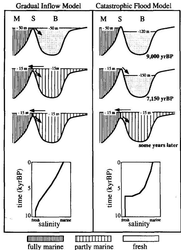
Fig. 5. Reconstructed levels in the Mediterranean ( M ) and Black Seas ( B ), and their connections/isolations via the SOÇ-Dardanelles and SOI-Bosporus sill ( S ). On the left is a portrayal of the gradual inflow model (Degens and Ross, 1972; Deuser, 1972, 1974) in which the first connection was made at 9000 yr BP. The depth of the strait deepened slowly as global eustatic sea level continued to rise, leading to an acceleration in the strengthening of the Black Sea's salinity. On the right is our catastrophic flood model in which the Mediterranean broke through a barrier in the inlet at 7150 yr BP and rapidly flooded a partly evaporated freshwater lake. Here increase in the Black Sea's salinity is shown to have been initially abrupt and then to have later decelerated.
