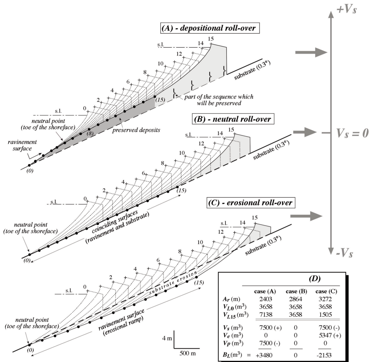
Fig. 7 - Comparative translation rates for the three types of roll-over under different conditions of sediment supply ( V_s ): (A) depositional roll-over with positive net supply ( V_s = 7500 m^3 for the total period); (B) neutral roll-over ( V_s = 0 ); (C) erosive roll-over ( V_s = -7500 m^3 for the total period). In (D), tabulated values for tracking parameter values: A_r = total littoral retreat; V_{L0-15} = volume of the littoral body at step 0 and 15; V_e and V_p = total sediment volume gained from substrate erosion ( V_e ) or lost from stratal preservation ( V_p ); B_L is the sedimentary balance on the littoral between steps 0 and 15.
