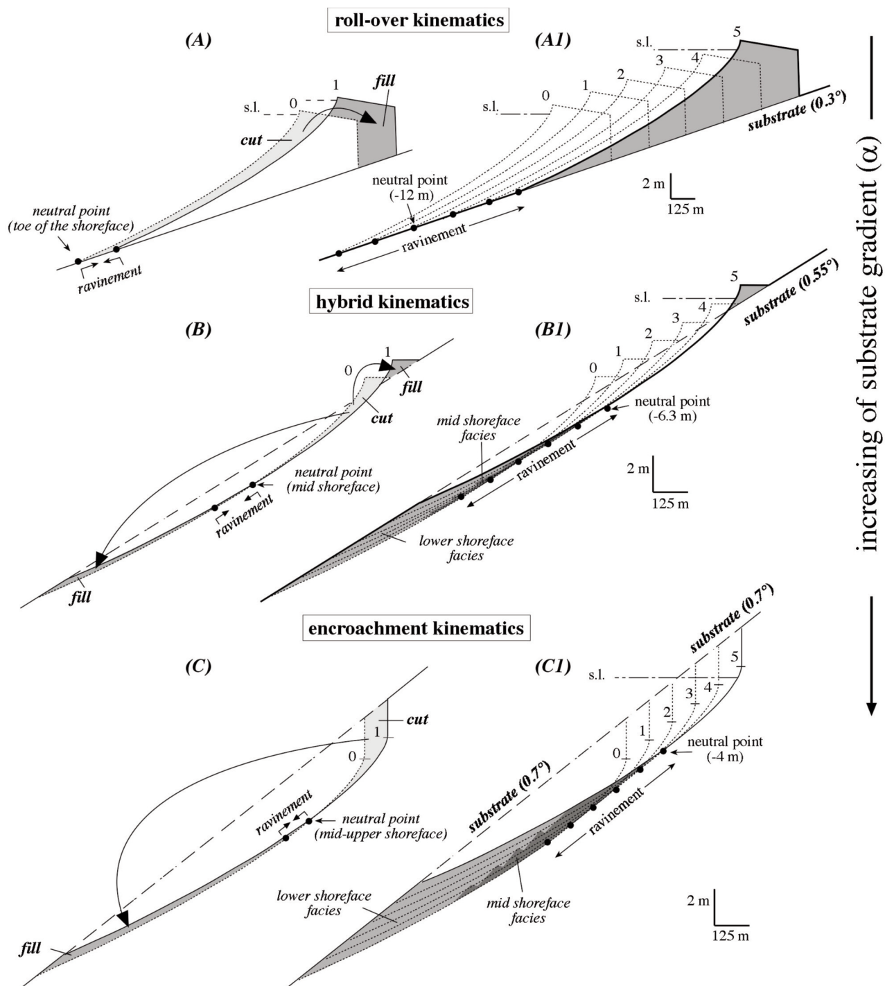
Fig. 3 - The three modes of coastal evolution during the sea level rise for different illustrative conditions of the ravine:shoreface gradient ratio (eq.1): (A) barrier roll-over; (B) hybrid translation; (C) encroachment (Cowell et al., 1995). The left-hand panel shows the fundamental geometric relationships between the shoreface and the substrate governing coastal accommodation and resulting sediment redistribution processes (arrows indicate sediment dispersal - cut to fill). Points in black indicate position of the "neutral point", translation of which produces a ravine surface. The right-hand panel shows distinctive stratigraphic architectures produced after multiple steps of each mode. Parameter values are the same for each mode ( V_s = 0 , V_f = 0 , L^* = 1150 m, h^* = 12 m, defined in Fig. 1); only the substrate slope differs and consequently the gradient ( \alpha ) of the ravine surface.
