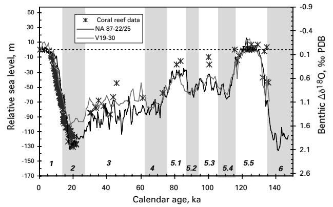
Fig. 1. Left axis: U-Th dated RSL estimates based on corals and other evidences (Bard et al., 1990a, b, 1996; Stein et al., 1993; Zhu et al., 1993; Gallup et al., 1994; Stirling et al., 1995; Chappell et al., 1996; Hanebuth et al., 2000; Yokoyama et al., 2000). Yokoyama's (2000) equivalent sea-level estimates have been converted into approximate RSL by subtracting 10 m. Right axis: North Atlantic patch of NA 87-22 and NA 87-25 \delta^{18}O_b relative to the modern \delta^{18}O_b value (3.32‰ PDB), and Pacific core V19-30 \delta^{18}O_b relative to the modern value (3.45‰ PDB), both versus calibrated 14 C ages until 40 kyr BP, and versus the SPECMAP time scale beyond (see Table 1 for cores location and references). Note that the SPECMAP time scale has been adjusted to be consistent with the U-Th dated RSL data at the transition between stages 6 and 5. Cibicides w. \delta^{18}O_b has been corrected by +0.64‰ to account for the difference in fractionation between this species and Uvigerina (Duplessy et al., 1984).
