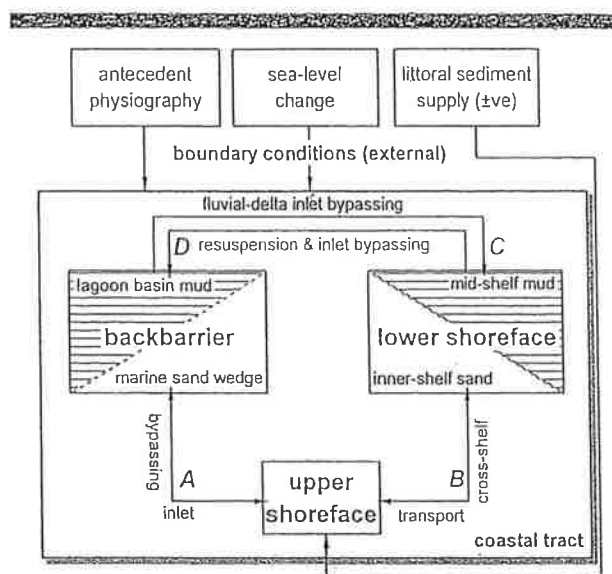
Figure 2. Schematic representation of mechanisms steering the location of the upper shoreface.
