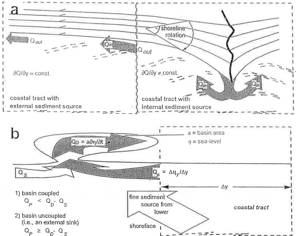
Figure 5. External and internal sources and sinks: a) Successive shorelines supplied by a river delta; and b) Estuarine basin as 1. dynamically-coupled sink, vs 2. external sink.
