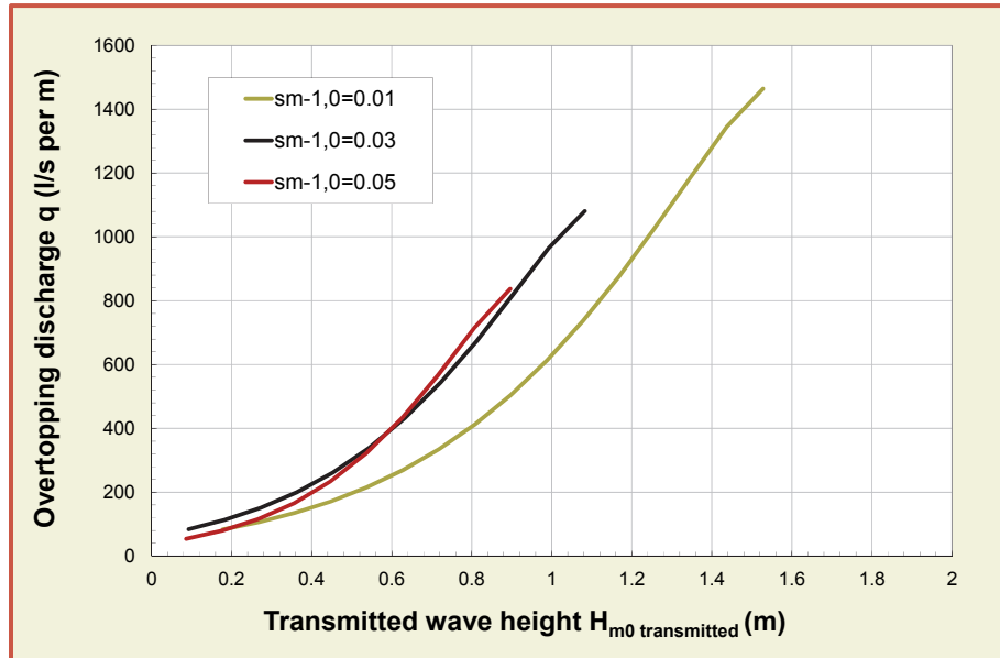
Figure 4.9: Wave transmission versus wave overtopping for a smooth 1:4 slope and a wave height of H_{m0} = 3 \text{ m}
