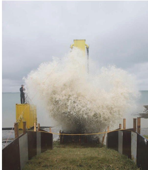
Figure 4.37 Measuring wave impacts on a 0.46 m high vertical step of a stair case, caused by run-up flows on a promenade from the wave run-up simulator
