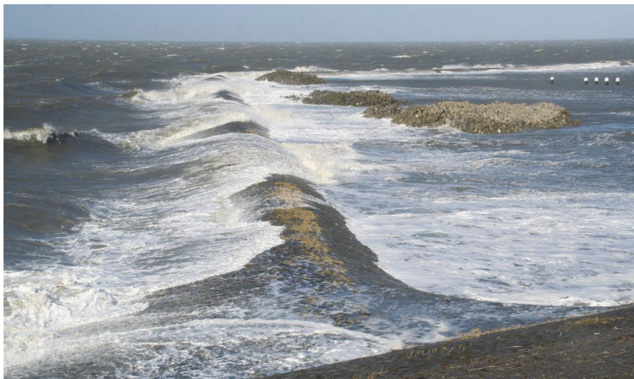
Figure 3.20 Dangerous overtopping over a smooth low-crested structure. Near locks at Afsluitdijk, NL
