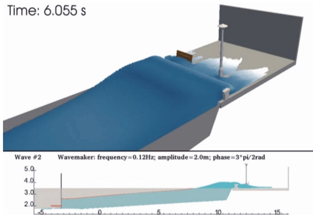
Figure 4.26: Numerical modelling results using the SPH solver DualSPHysics for a dike with a storm wall. The geometries of the bed, the dike and the road with storm wall are shown. At a particular time instant, the simulated wave overtopping has been visualised in a 2D slice and in a 3D picture, to illustrate the 3D flow processes. Courtesy of A. Crespo
