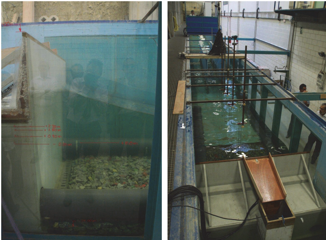
Figure 4.28: Cross-section of a vertical caisson in a wave flume (left) with the overtopping chute and tank (right). Wave flume at INHA, ES
