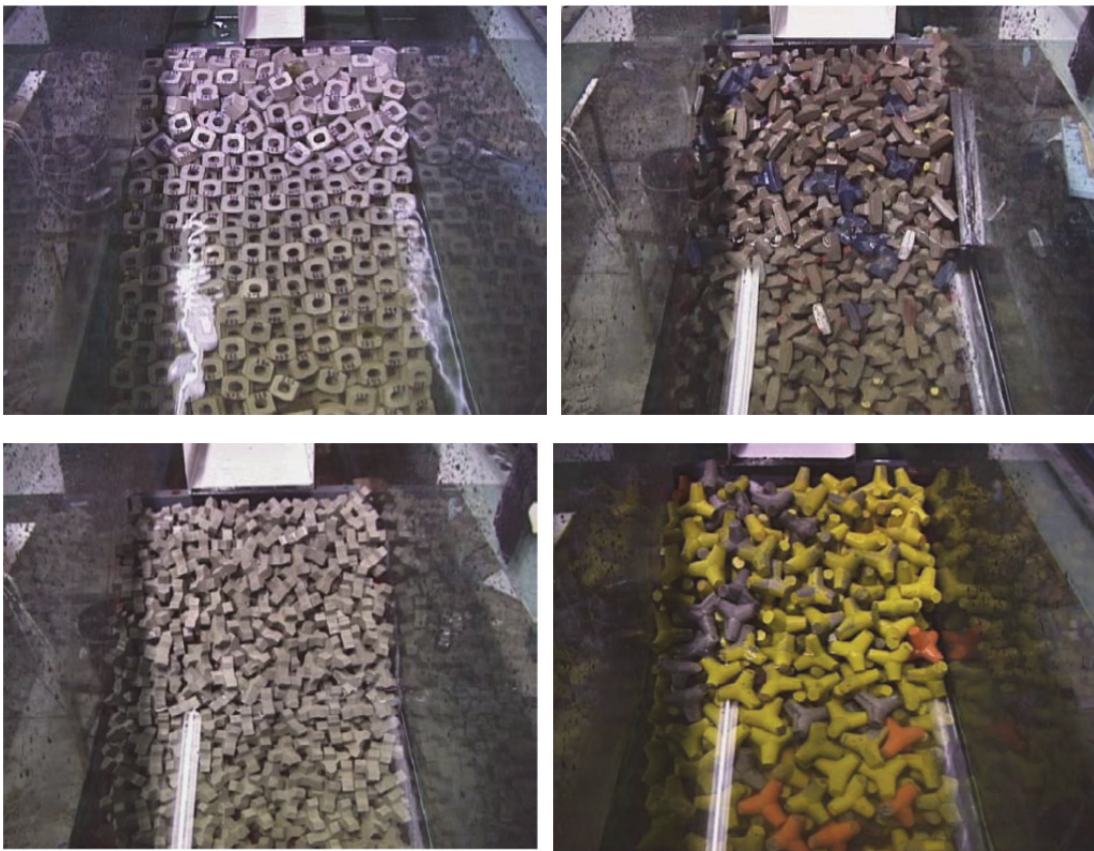
Figure 6.9: Clockwise from top left: Haros, Accropode I, Xbloc and Tetrapods; Test set-up in CLASH
