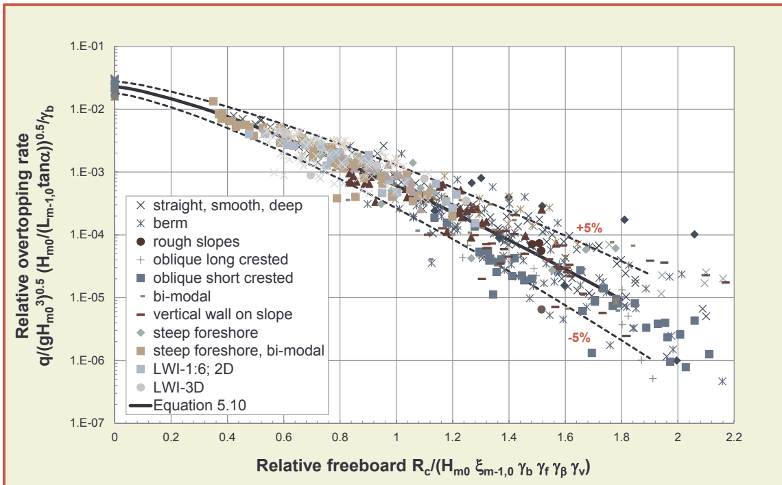
Figure 5.12: Wave overtopping data for breaking waves and overtopping Equation 5.10 with 5% under and upper exceedance limits (= 90%-confidence band)
