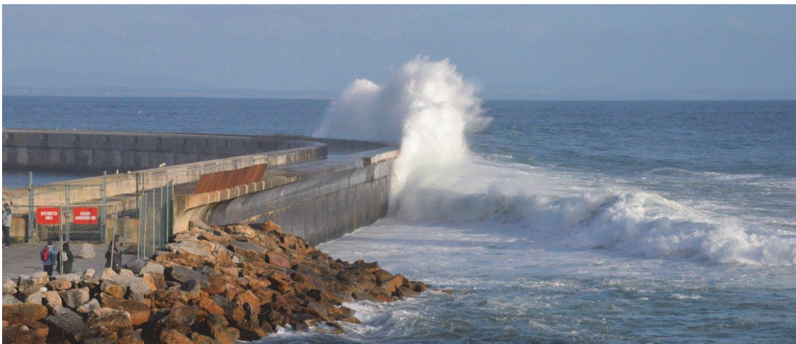
Figure 1.8: Effective fairly significant bullnose at Cascais, Portugal. Waves are breaking on the foreshore and give impulsive wave conditions. There was no wind. Courtesy L. Franco
