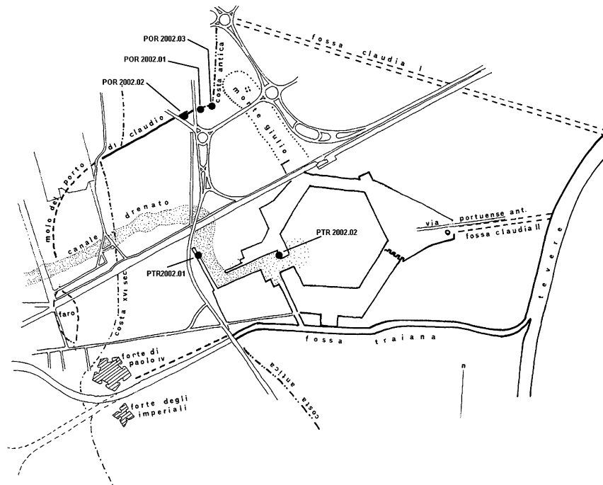
Figure 10. Portus, plan of Roman harbour with indication of core locations.
