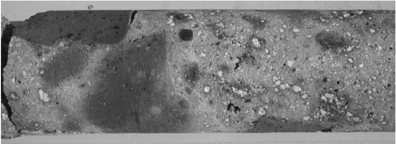
Figure 15. Core SLI.2003.01, area around -0.78 m.
