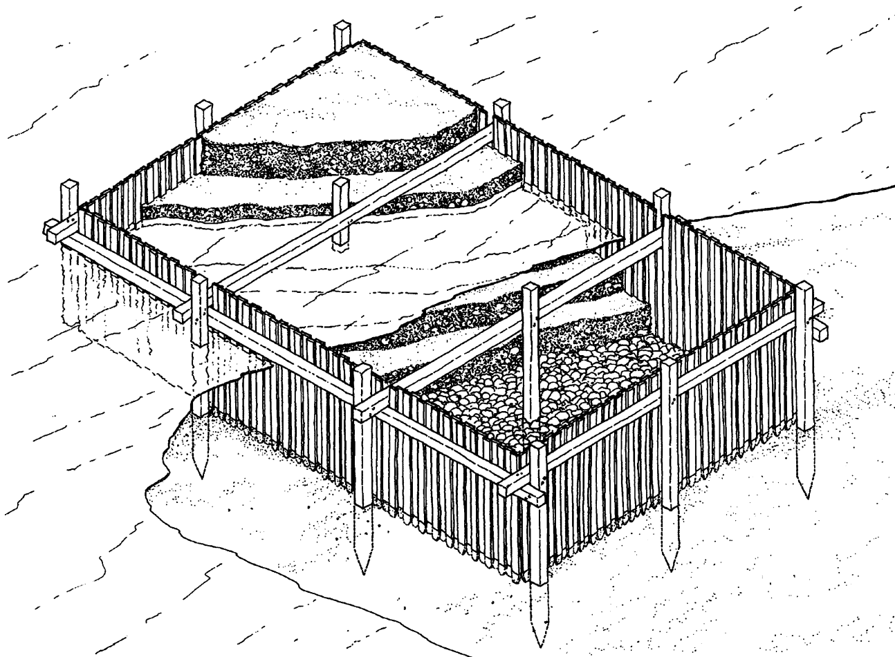
Figure 1. Vitruvius' formwork for hydraulic concrete. Reconstruction. (C. Brandon)
