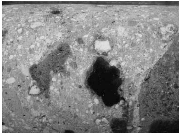
Figure 6. Core POR.2002.02, detail at –1.75 m.
