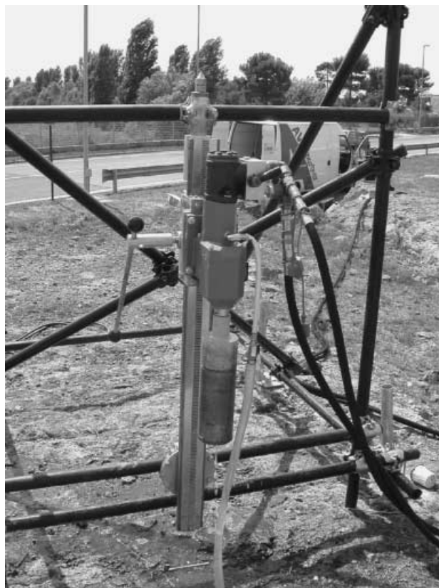
Figure 7. Coring motor and rack, detail.
