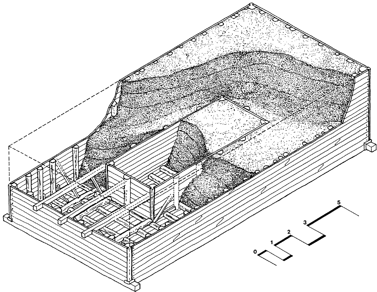
Figure 5. Caesarea: single-use barge formwork. Reconstruction. (C. Brandon)
