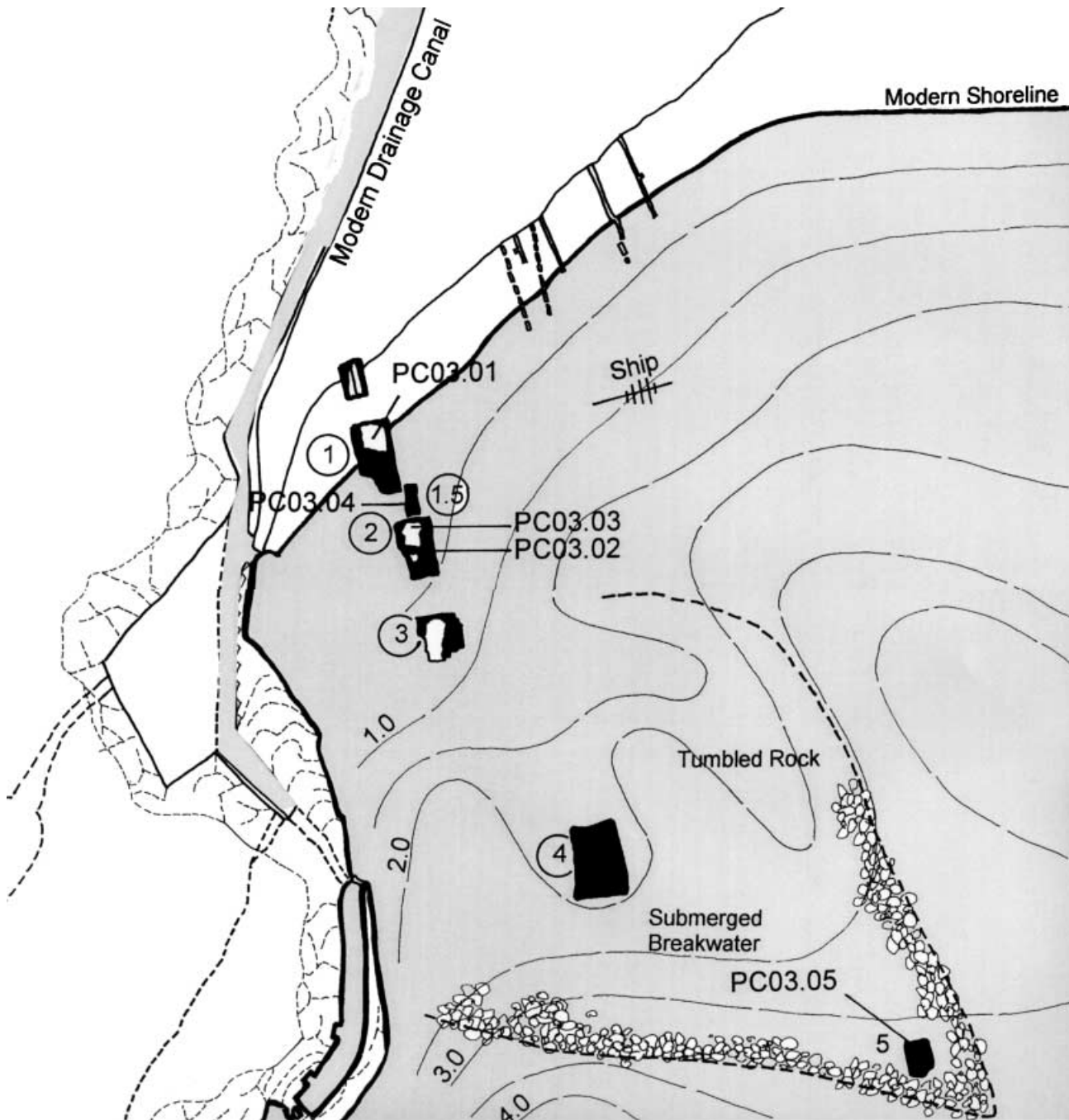
Figure 3. Cosa: Plan of outer harbour with coring locations (after McCann et al. , 1987).
